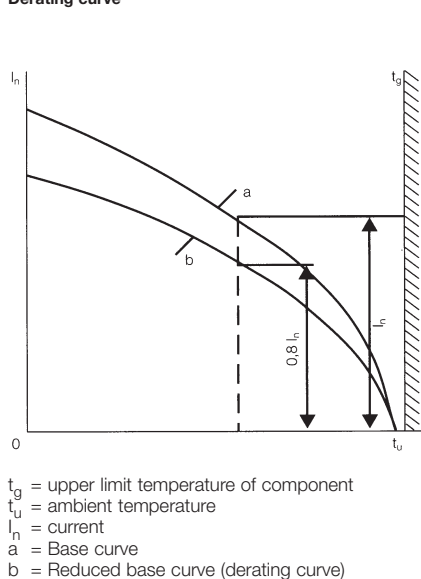
Derating curve
