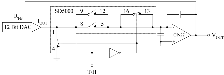
Figure 21. DAC Deglitcher Using DMOS Switches
