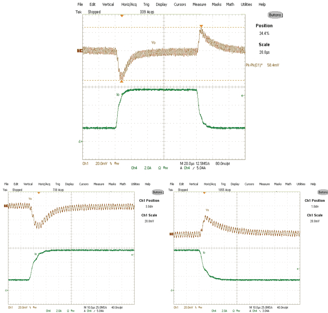
Fig. 28: Transient Response 1.4A(10%)-5.6A(40%) load (0.5A/μs) Ch_1:V_{out} , Ch_4:I_o
