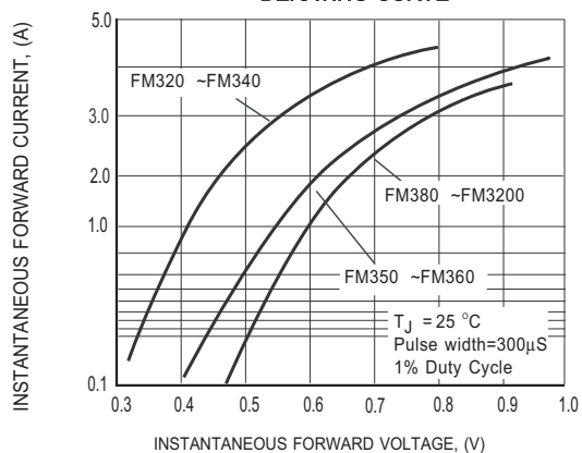
FIG.3 MAXIMUM INSTANTANEOUS FORWARD CHARACTERISTICS
