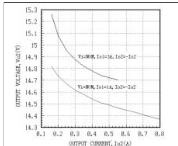
Fig. 26 AEW05ACC48 Load Regulation Curves T_c=25^{\circ}\text{C}
