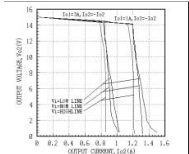
Fig. 22 AEW05ACC48 Auxiliary output Character Curves
