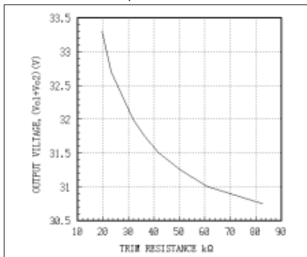
Fig. 41 AEW 15V Dual Output Trim Up Curve Rated input, rated load, T_c=25^\circ\text{C}
