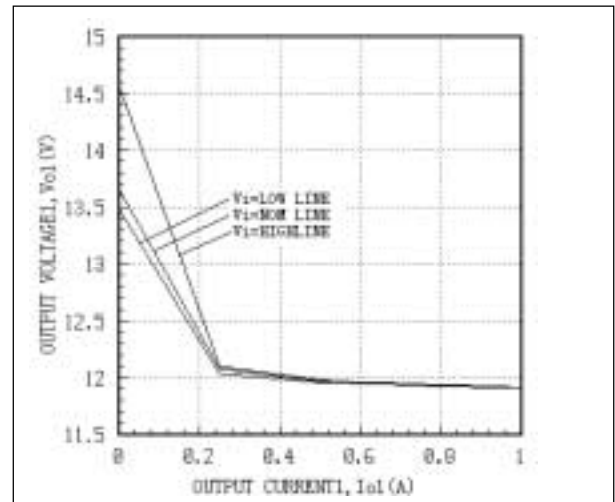
Fig. 26 AEW01BB24 Load Regulation Curves I_{o2}=10\%I_o constant, I_{o1} variable, T_c=25^\circ\text{C}
