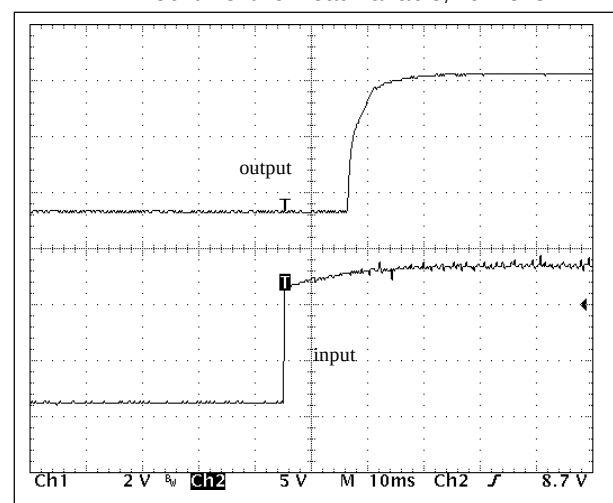
Fig. 6 Output voltage rise up (AV30-48T0512 typ.) current signal on CNT, I_o=80\%I_{o,max} , T_c=25^\circ\text{C}
