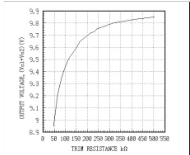
Fig. 38 AEW 5V Dual Output Trim Down Curve Rated input, rated load, T_c=25^\circ\text{C}
