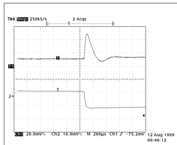
Fig. 4 Dynamic Response 50%-75% I_{o1} load variable, T_c=25^\circ\text{C}
