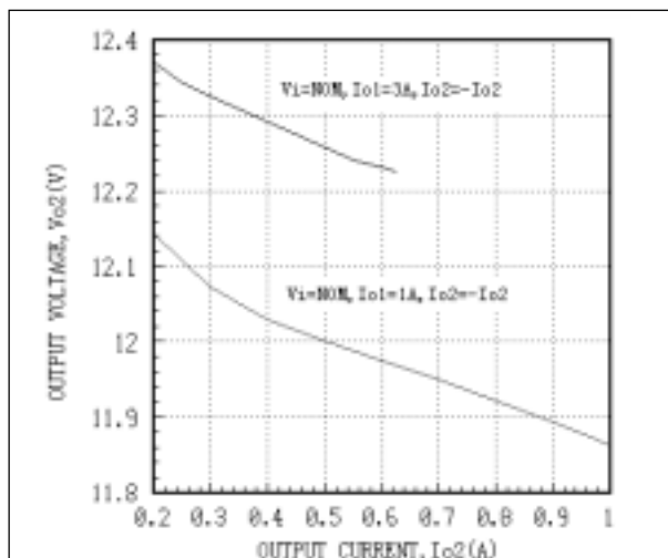
Fig. 23 AEW05ABB24 Load Regulation Curves
