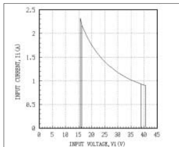
Fig. 12 AEW05ACC24 Input Characteristic Curves T_c = 25^\circ\text{C}
