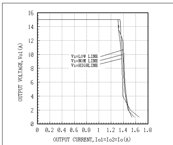
Fig. 21 AEW01CC24 Output Overcurrent Curves
