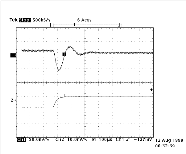
Fig. 43 Dynamic Response 50%-75% load variable, Tc=25°C
