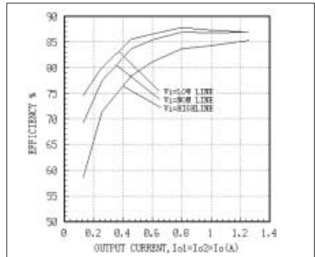
Fig. 8 AEW01BB24 Efficiency Curves
