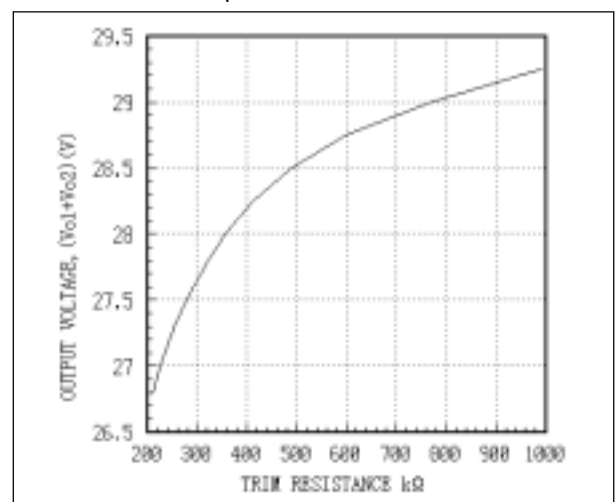
Fig. 42 AEW 15V Dual Output Trim Down Curve Rated input, rated load, T_c=25^\circ\text{C}
