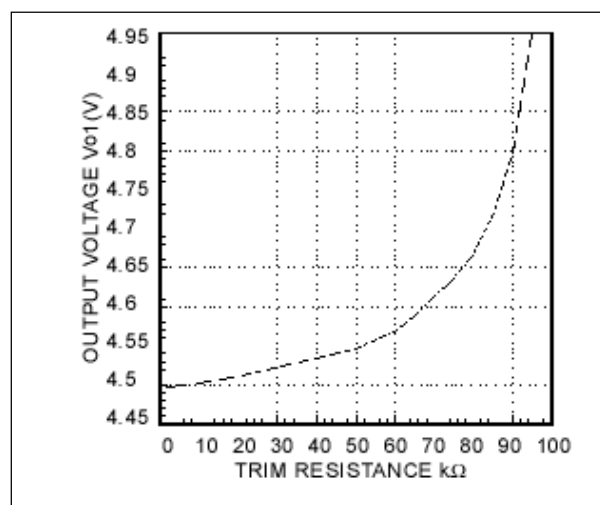
Fig. 32 AV30-*T* Trim Down Rated voltage, rated current, Tc=25°C
