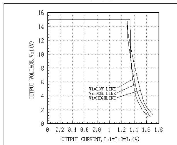
Fig. 24 AEW01CC48 Output Overcurrent Curves
