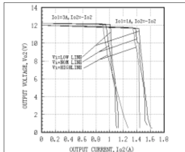
Fig. 16 AEW05ACC24 Auxiliary output Character Curves
