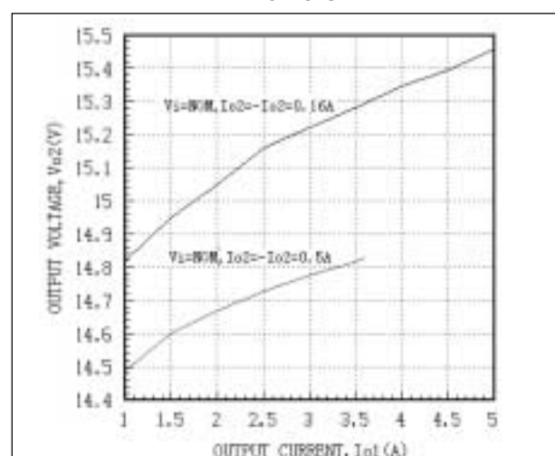
Fig. 30 AEW05ACC48 Cross Regulation Curves T_c=25^{\circ}\text{C}
