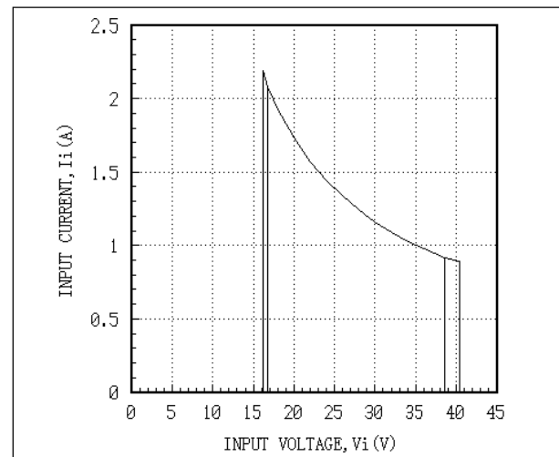
Fig. 14 AEW01BB24 Input Characteristic Curves
