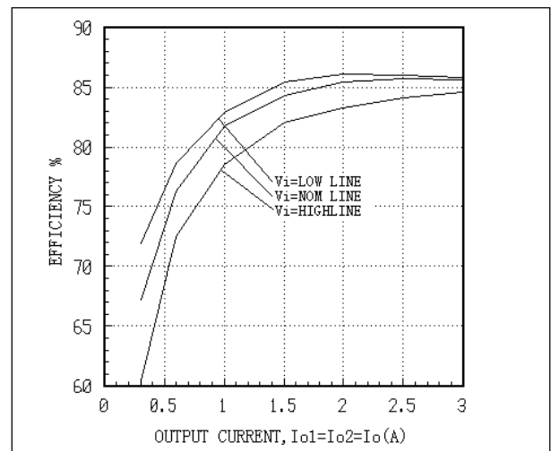
Fig. 10 AEW03AA48 Efficiency Curves
