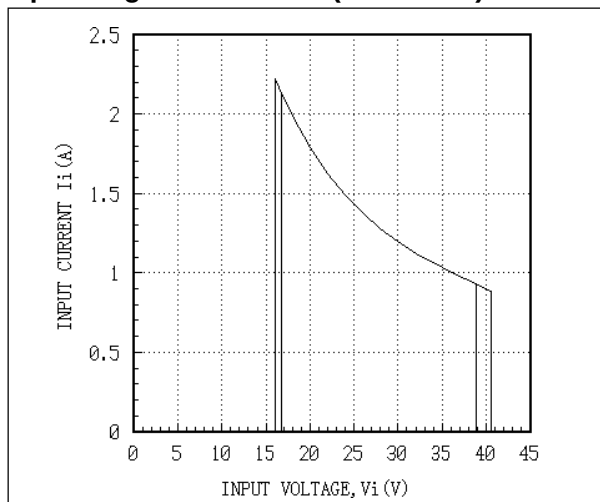
Fig. 13 AEW03AA24 Input Characteristic Curves
