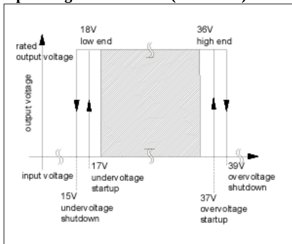
Fig. 1 24V input voltage range (typ.)
