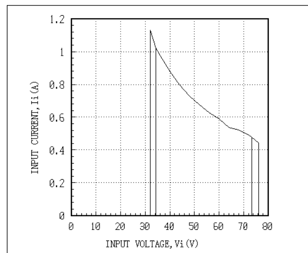
Fig. 16 AEW03AA48 Input Characteristic Curves
