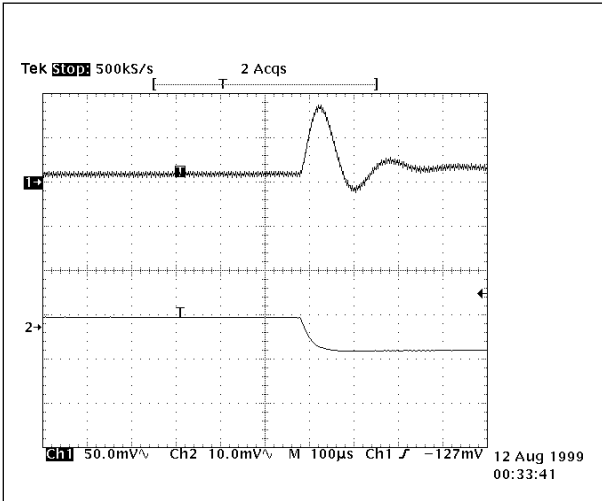
Fig. 44 Dynamic Response 50%-75% load variable, Tc=25°C
