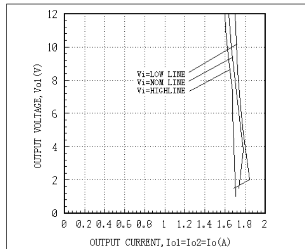
Fig. 20 AEW01BB24 Output Overcurrent Curves
