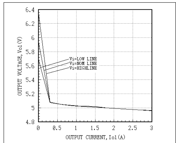
Fig. 28 AEW03AA48 Load Regulation Curves I_{o2}=10\%I_o constant, I_{o1} variable, T_c=25^\circ\text{C}
