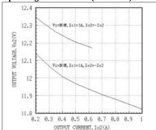
Fig. 25 AEW05ABB48 Load Regulation Curves T_c=25^{\circ}\text{C}
