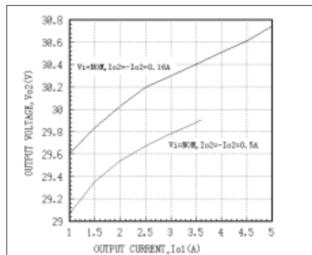
Fig. 28 AEW05ACC24 Cross Regulation Curves T_c=25^{\circ}\text{C}
