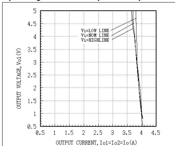
Fig. 19 AEW03AA24 Output Overcurrent Curves
