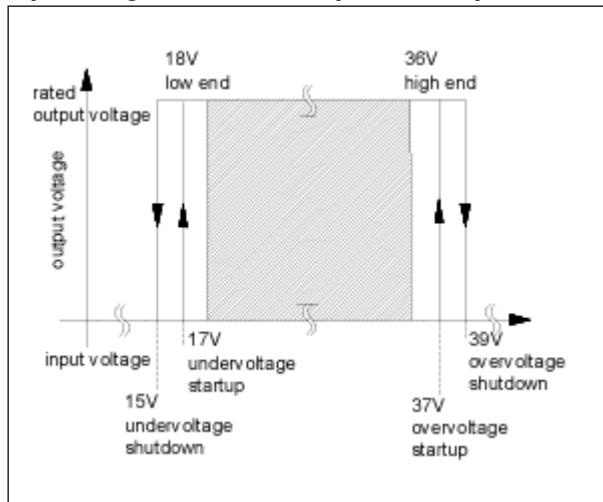
Fig. 1 24V input voltage range (typ.)
