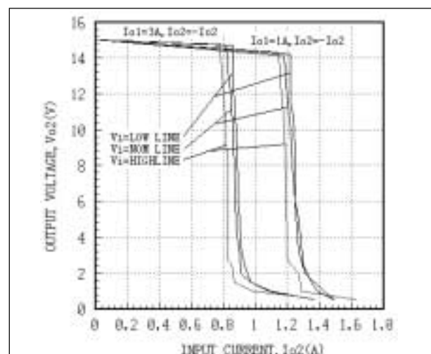
Fig. 18 AEW05ACC48 Auxiliary output Character Curves
