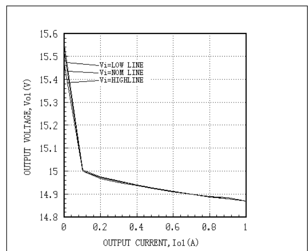
Fig. 30 AEW01CC48 Load Regulation Curves I_{o2}=10\%I_o constant, I_{o1} variable, T_c=25^\circ\text{C}
