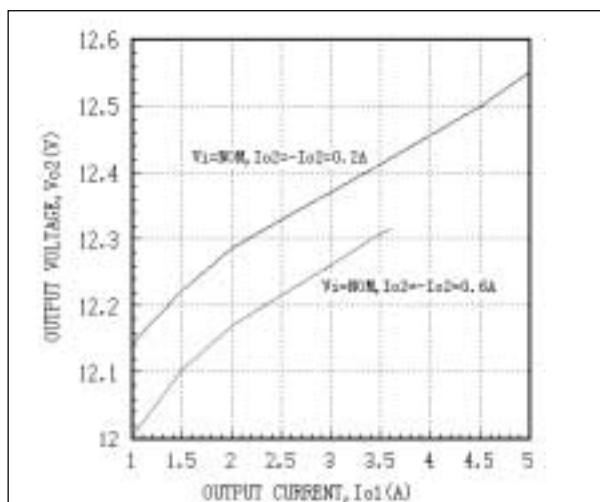
Fig. 27 AEW05ABB24 Cross Regulation Curves T_c=25^{\circ}\text{C}
