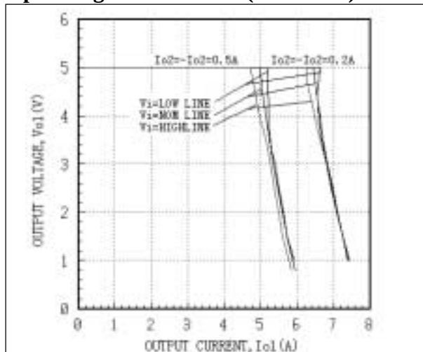
Fig. 19 AEW05ABB24 Main Output Character Curves
