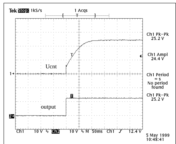
Fig. 6 output voltage rise up curve (rated voltage, current signal on CNT, I_o=80\%I_{o,max} , T_c=25^\circ\text{C} )
