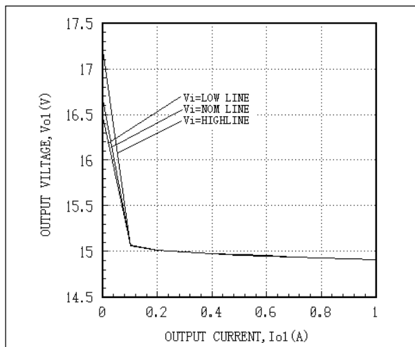
Fig. 27 AEW01CC24 Load Regulation Curves I_{o2}=10\%I_o constant, I_{o1} variable, T_c=25^\circ\text{C}
