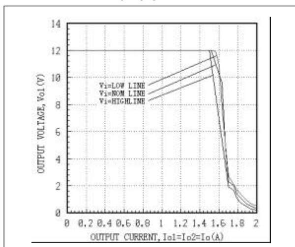
Fig. 23 AEW01BB48 Output Overcurrent Curves
