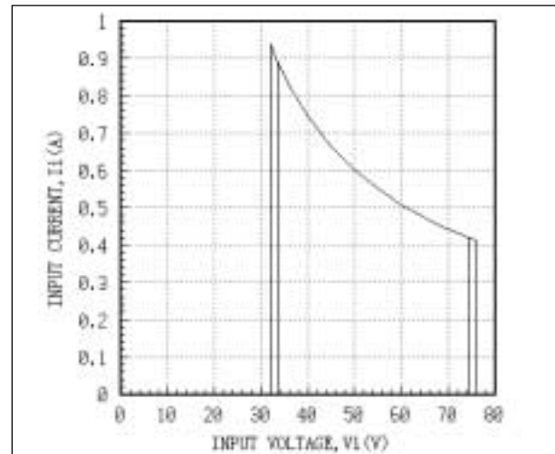
Fig. 14 AEW05ACC48 Input Characteristic Curves
