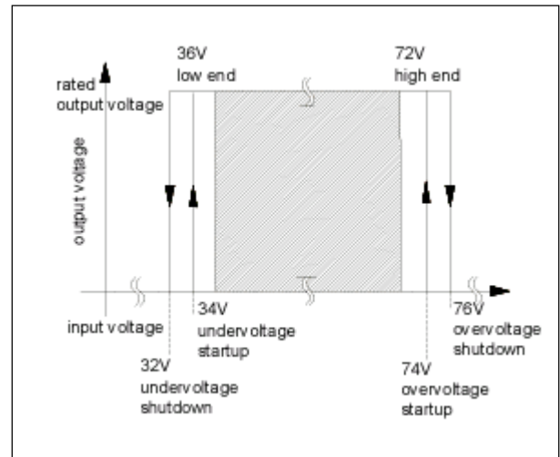
Fig. 2 48V input voltage range (typ.)
