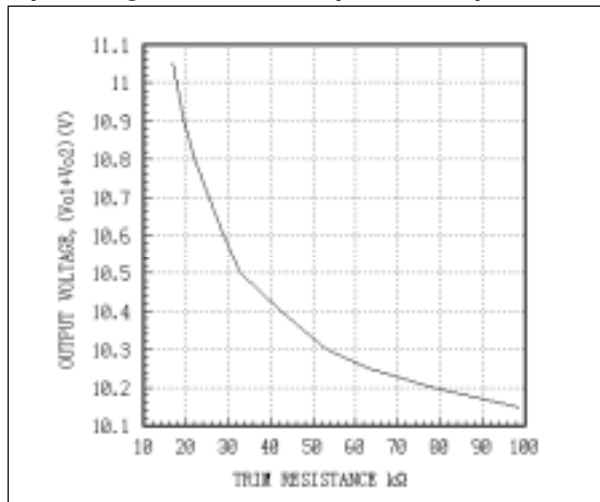
Fig. 37 AEW 5V Dual Output Trim Up Curve Rated input, rated load, T_c=25^\circ\text{C}
