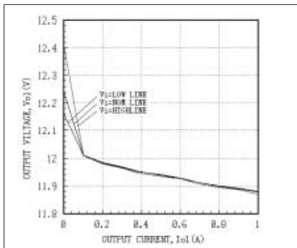
Fig. 29 AEW01BB48 Load Regulation Curves I_{o2}=10\%I_o constant, I_{o1} variable, T_c=25^\circ\text{C}
