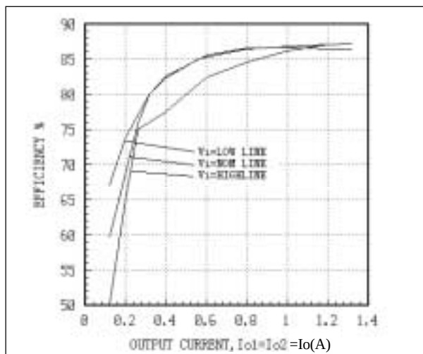
Fig. 11 AEW01BB48 Efficiency Curves
