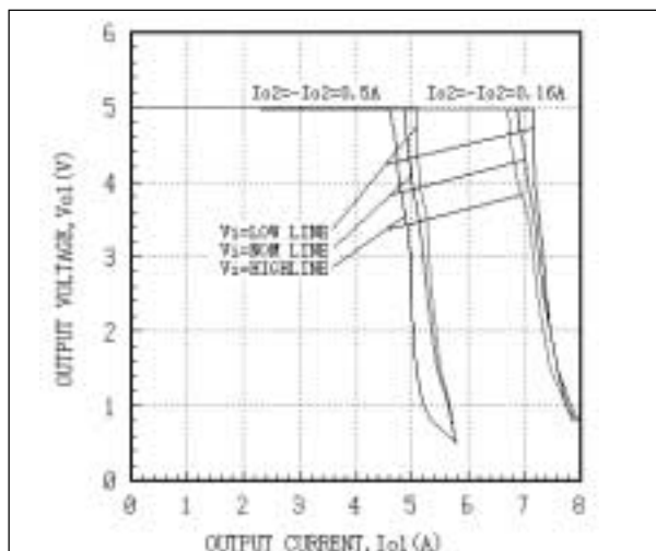
Fig. 17 AEW05ABB48 Main Output Character Curves
