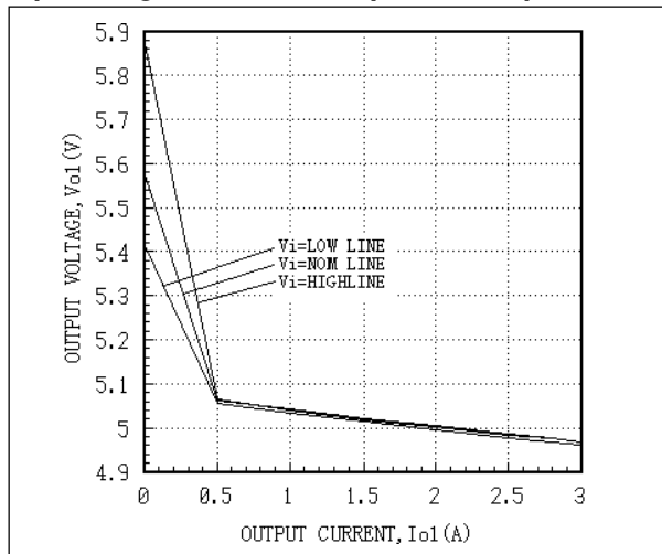
Fig. 25 AEW03AA24 Load Regulation Curves I_{o2}=10\%I_o constant, I_{o1} variable, T_c=25^\circ\text{C}
