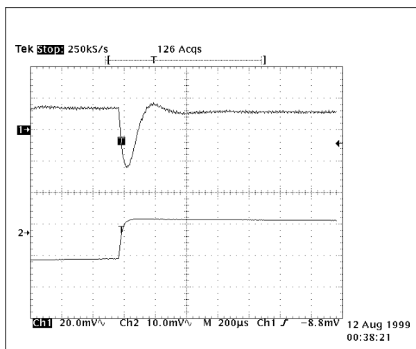
Fig. 3 Dynamic Response 50%-75% I_{o1} load variable, T_c=25^\circ\text{C}
