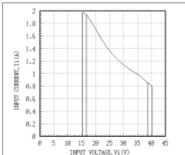
Fig. 11 AEW05ABB24 Input Characteristic Curves T_c = 25^\circ\text{C}
