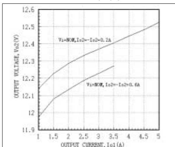
Fig. 29 AEW05ABB48 Cross Regulation Curves T_c=25^{\circ}\text{C}
