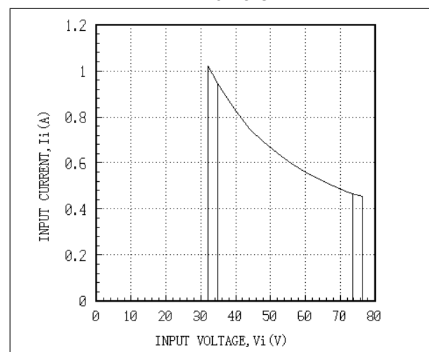
Fig. 18 AEW01CC48 Input Characteristic Curves
