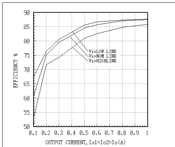
Fig. 9 AEW01CC24 Efficiency Curves
