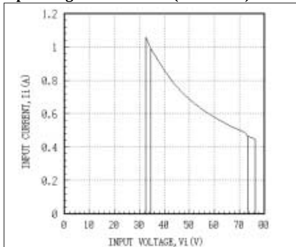
Fig. 13 AEW05ABB48 Input Characteristic Curves
