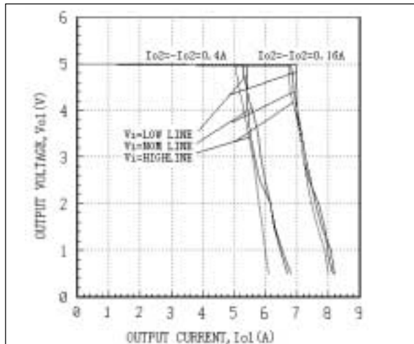
Fig. 21 AEW05ABB48 Main Output Character Curves
