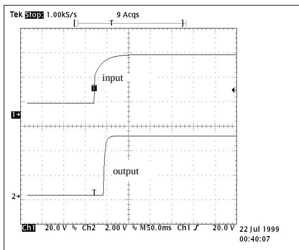
Fig. 5 Output voltage rise up curve (Power on character, I_o=80\%I_{o,max} , T_c=25^\circ\text{C} )
