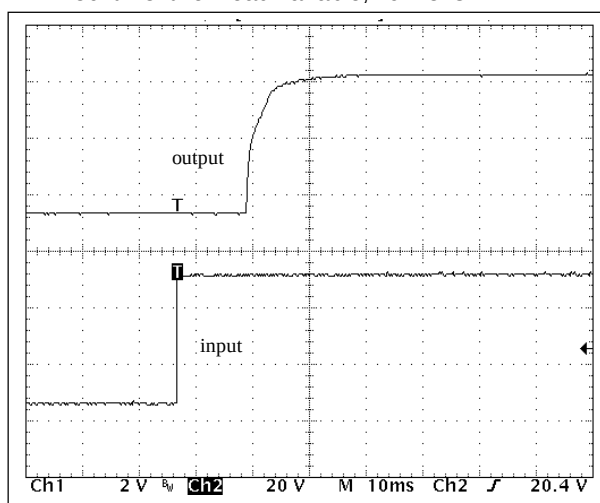
Fig. 5 Output voltage rise up (AV30-48T0512 typ.) (Power on character, I_o=80\%I_{o,max} , T_c=25^\circ\text{C} )
