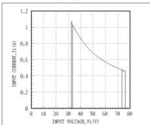
Fig. 17 AEW01BB48 Input Characteristic Curves
