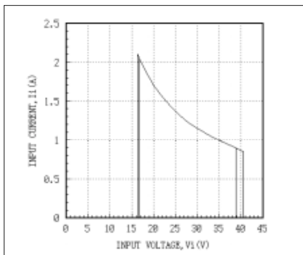
Fig. 15 AEW01CC24 Input Characteristic Curves
