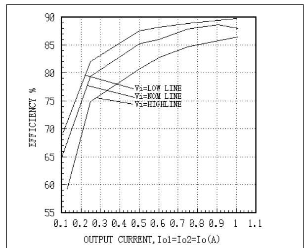
Fig. 12 AEW01CC48 Efficiency Curves
