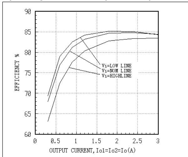
Fig. 7 AEW03AA24 Efficiency Curves
