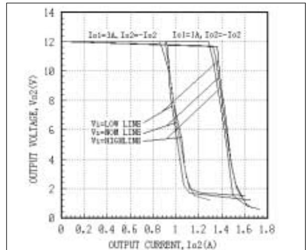
Fig. 20 AEW05ACC24 Auxiliary output Character Curves
