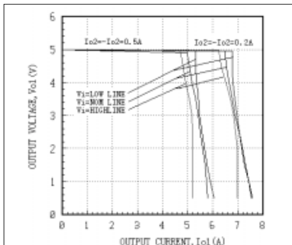
Fig. 15 AEW05ABB24 Main Output Character Curves
