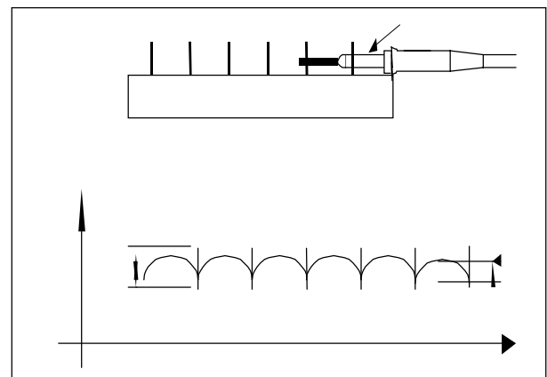
Fig. 4 Output ripple & noise testing method
