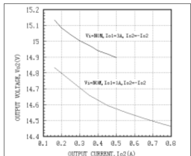
Fig. 24 AEW05ACC24 Load Regulation Curves
