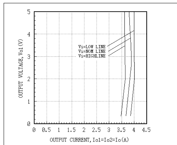
Fig. 22 AEW03AA48 Output Overcurrent Curves
