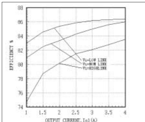
Fig. 9 AEW05ABB48 Efficiency Curves I_{o2} = -I_{o2} = I_o , min T_c = 25^\circ\text{C}
