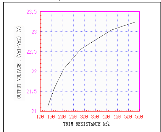
Fig. 40 AEW 12V Dual Output Trim Down Curve Rated input, rated load, T_c=25^\circ\text{C}
