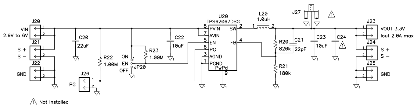
Figure 2. TPS62067EVM Schematic
