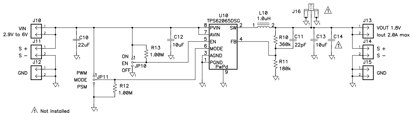
Figure 1. TPS62065EVM Schematic
