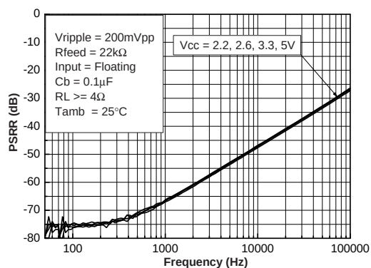
Figure 13. PSRR vs. power supply R_{feed} = 22 k\Omega
