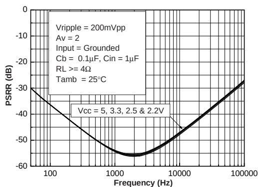
Figure 12. PSRR vs. power supply C_b = 0.1 \mu F , C_{in} = 1 \mu F
