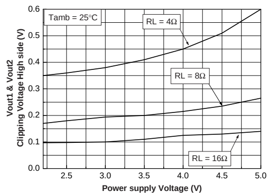
Figure 36. Clipping voltage vs. power supply voltage and load resistor T_{amb} = 25^\circ\text{C}
