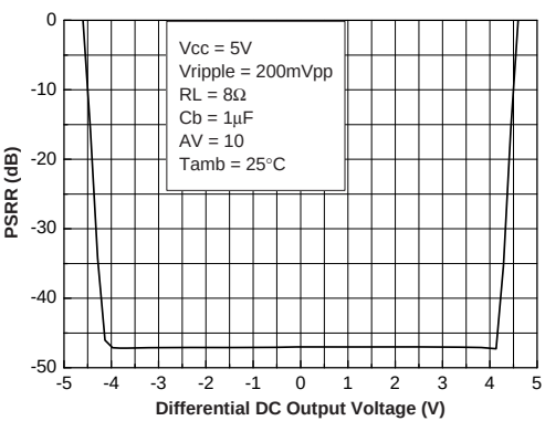
Figure 15. PSRR vs. DC output voltage A_V = 10
