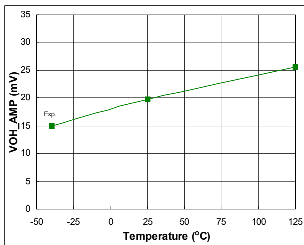
Fig. 73. Operational Amplifier Low Level Output Voltage vs. Temperature
