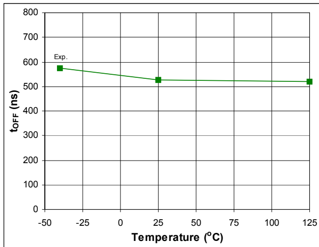
Fig. 43. Turn-off Propagation Delay vs. Temperature
