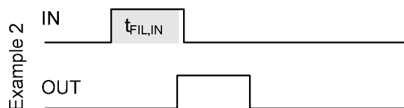
Figure 13: Advanced input filter
