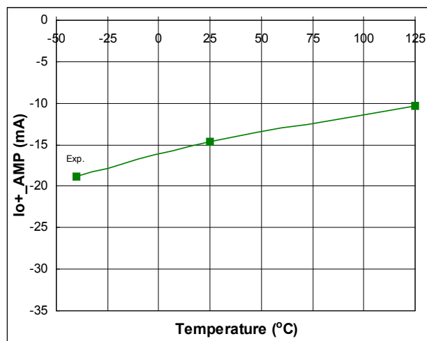
Fig. 77. Operational Amplifier Output High Short Circuit Current vs. Temperature
