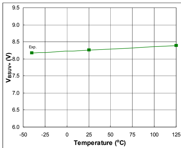
Fig. 65. V_{BS} Supply Undervoltage Positive Going Threshold vs. Temperature
