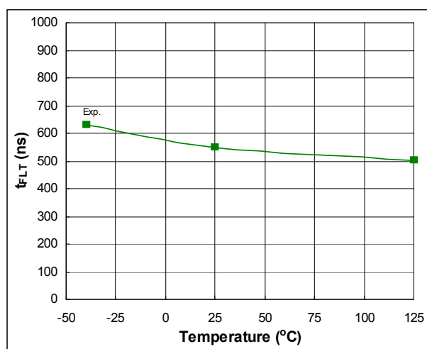
Fig. 47. ITRIP to FAULT Indication Delay vs. Temperature
