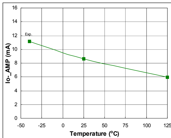
Fig. 75. Operational Amplifier Output Low Short Circuit Current vs. Temperature
