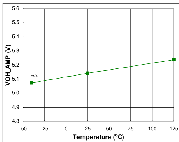
Fig. 72. Operational Amplifier High Level Output Voltage vs. Temperature
