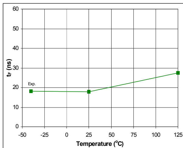
Fig. 45. Turn-off Fall Time vs. Temperature
