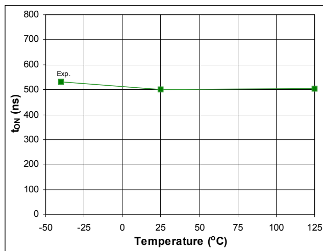
Fig. 41. Turn-on Propagation Delay vs. Temperature
