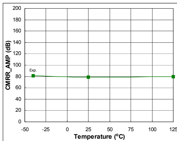
Fig. 71. Operational Amplifier Common Mode Rejection Ratio vs. Temperature
