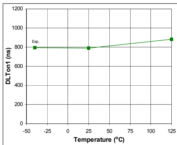
Fig. 49. Dead Time vs. Temperature
