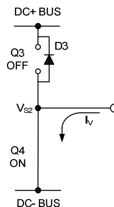
Figure 24: Q4 conducting
