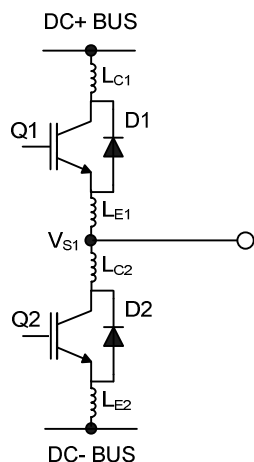
Figure 25: Parasitic Elements
