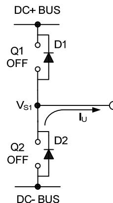
Figure 22: D2 conducting
