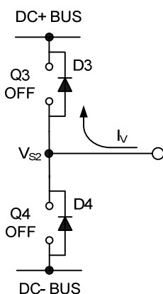
Figure 23: D3 conducting
