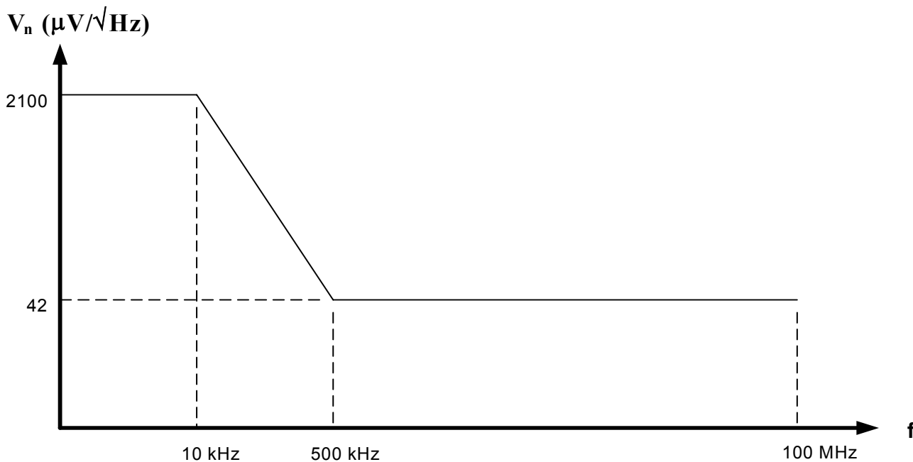
Figure 10. Power Supply Noise Tolerance Mask
