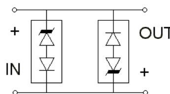
FIGURE 4 Optional Bidirectional configuration (two TVS devices in anti-parallel)
