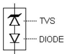
FIGURE 2 TVS with internal Low Capacitance Diode
