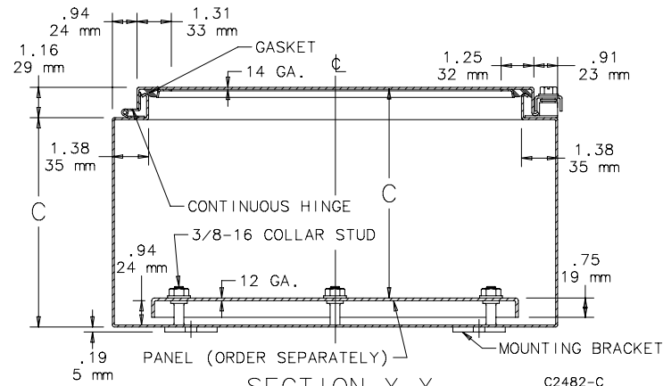
SECTION X-X
