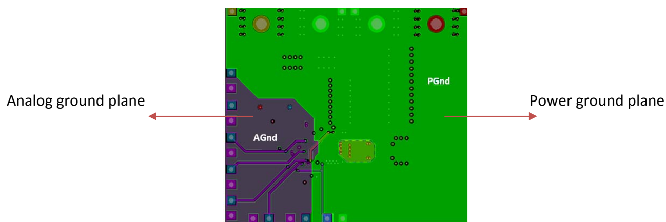
Figure 47c: IRDC3894 Demo board Layout Considerations – Mid Layer 1
