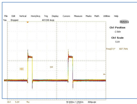
Figure 34: Inductor node at 12A load, Ch1:SW node
