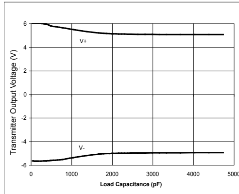
SP3225E/SP3227E Transmitter Output Voltage
