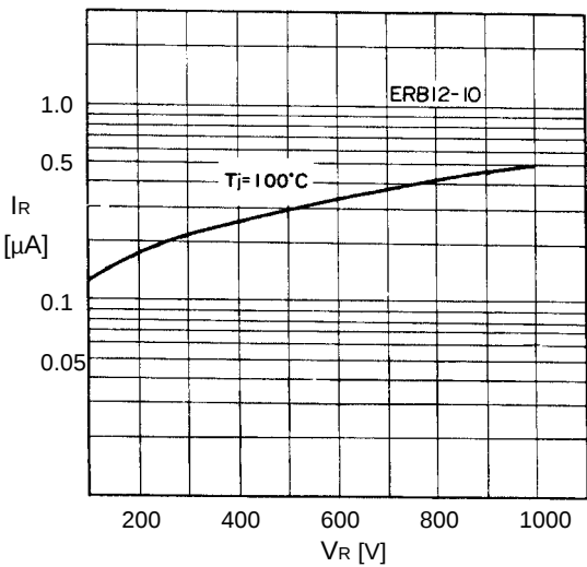
Reverse characteristics
