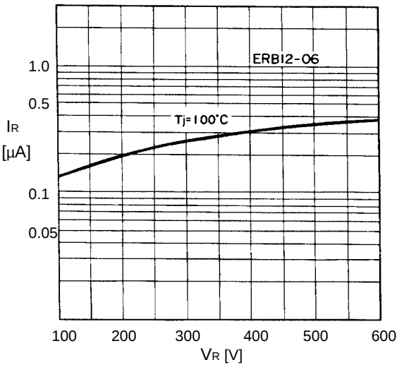
Reverse characteristics
