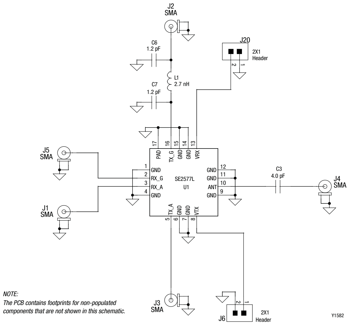
Figure 3. SE2577L Suggested Application Schematic
