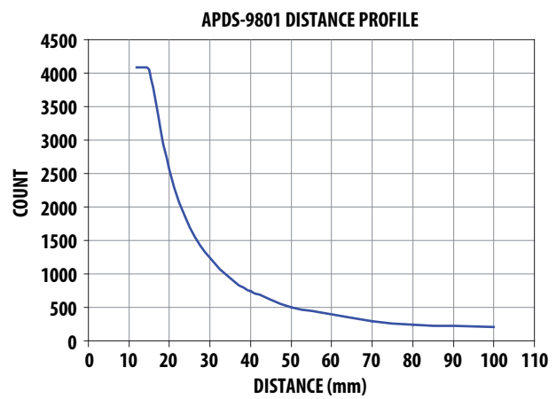
Figure 6. PS Output vs. Distance Typical Profile
