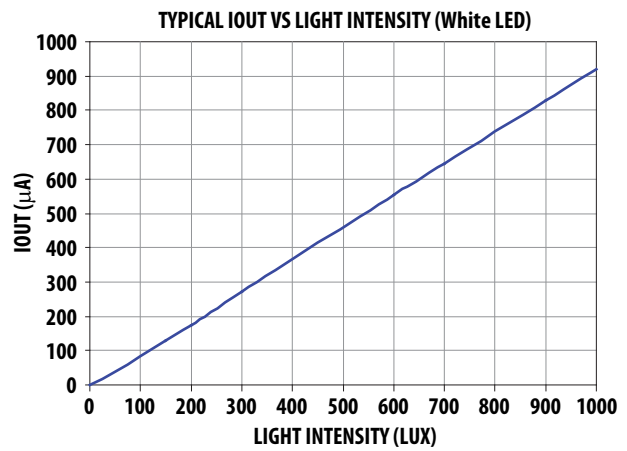
Figure 4. ALS Typical Output Current vs. Light Intensity
