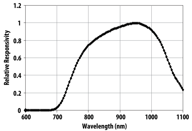
Figure 2. PS Photo Detector Spectral Response
