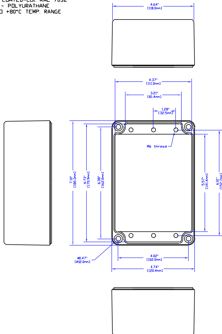
VIEW OF BOX (LID REMOVED)
