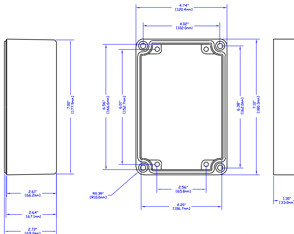
VIEW OF LID (INSIDE)
