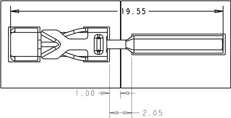
BTB MATING WITH RECEPTACLE P/N:2834167-3
