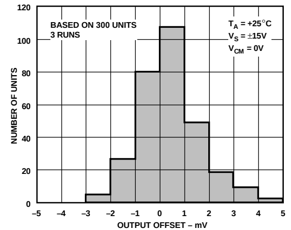
Figure 21. Output Offset ( V_{oos} ) Distribution @ \pm 15 V
