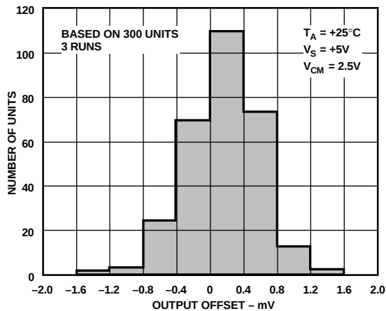
Figure 20. Output Offset ( V_{oos} ) Distribution @ +5 V
