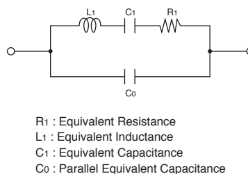
Fig. 2-3 Electrical Equivalent Circuit of CERALOCK®
