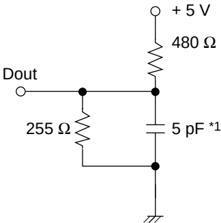
Output load (B)
