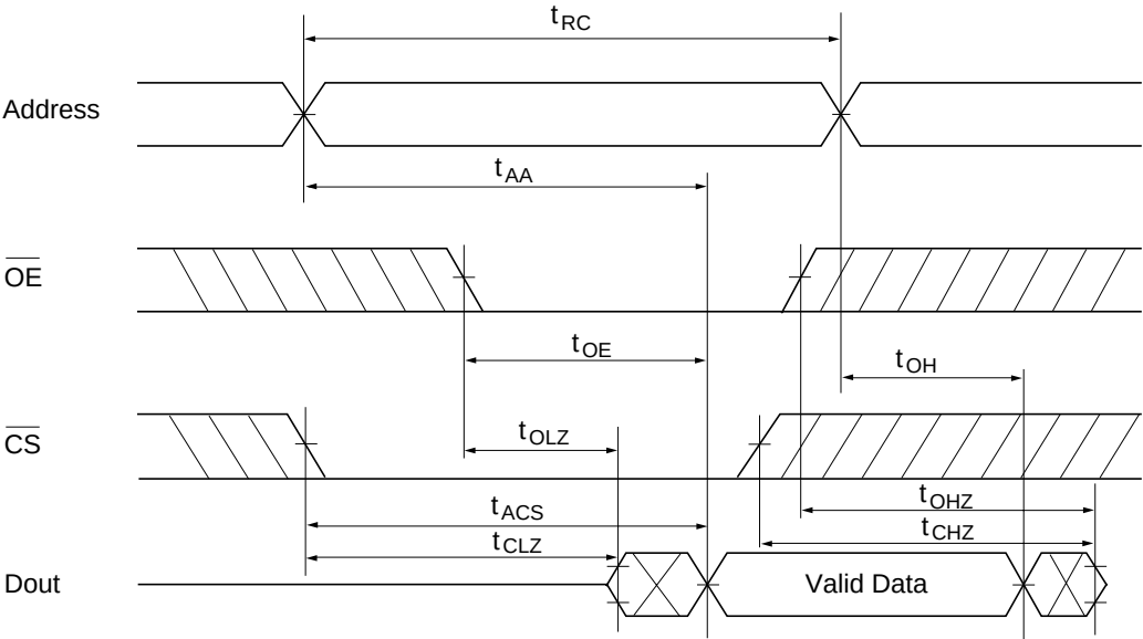
Read Timing Waveform (1)*1 ( \overline{WE} = V_{IH} )
