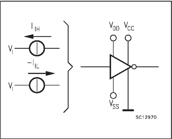
FIGURE 2: Driver Test Circuit for I IH and I IL
