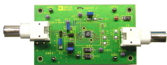
Figure 32. AD737 Evaluation Board
