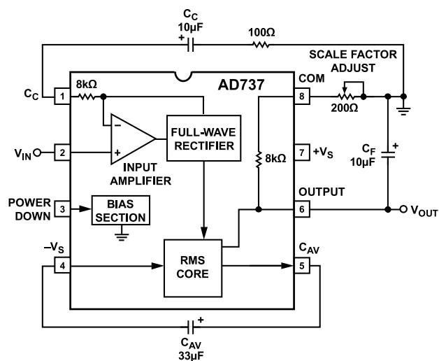
Figure 29. External Scale Factor Trim
