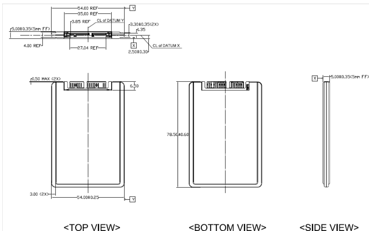
[Figure 2-1] Physical dimension
