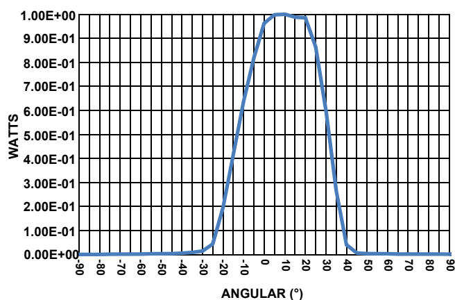
FIGURE 12. RADIATION EMISSION PATTERN IRLED TRANSVERSE
