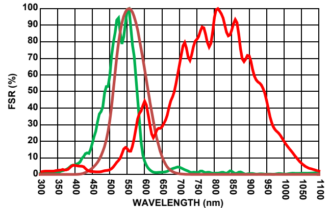
FIGURE 5. ISL29044 SENSITIVITY TO DIFFERENT WAVELENGTHS
