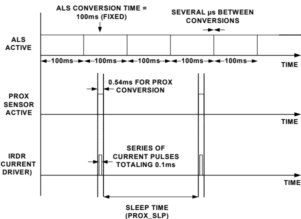
FIGURE 15. TIMING DIAGRAM FOR PROX/ALS EVENTS - NOT TO SCALE
