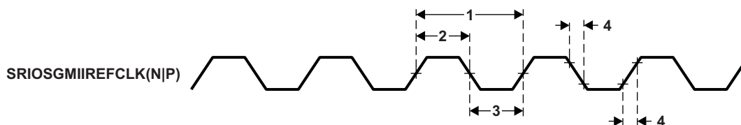
Figure 7-43. SRIOSGMIIREFCLK(N|P) Timing
