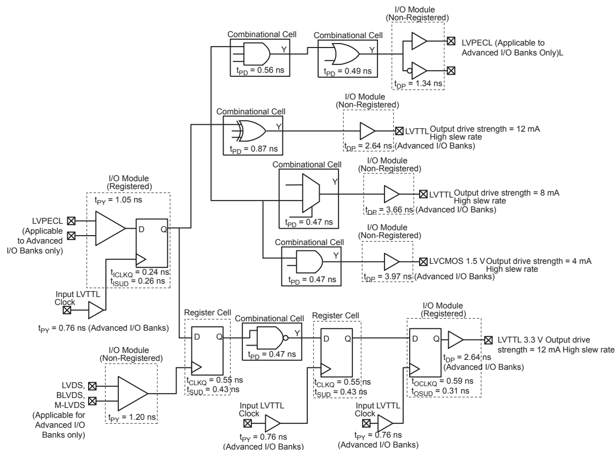
Figure 2-2 • Timing Model
