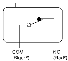
SPST-NC
