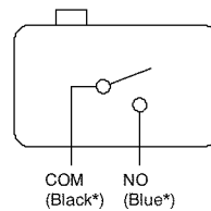
SPST-NO
