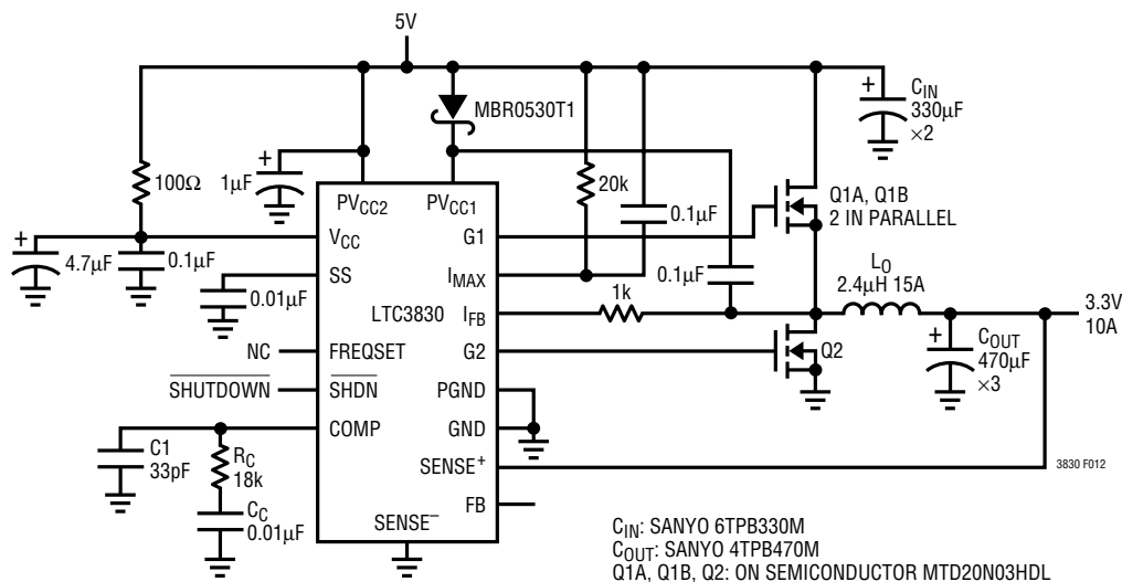
Figure 12. Typical 5V to 3.3V, 10A Application
