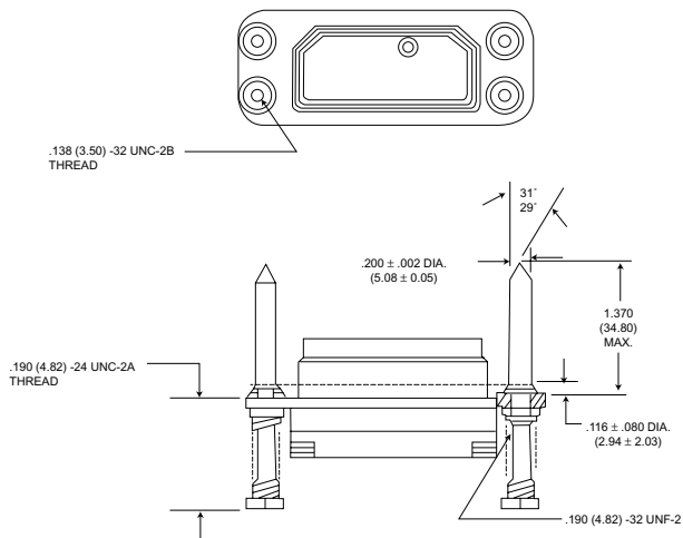
Mounting Style X - MIL-C-83733/2(USAF) With Guide Pins and Spring Mounting
