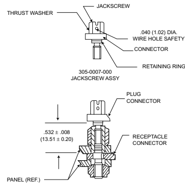
Mounting Spacing Dimensions For Jackscrew Assemblies
