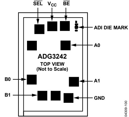
Figure 3. Die Pad Configuration (Die size: 550 μm × 820 μm)
