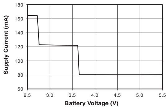
Supply Current vs Battery Voltage
