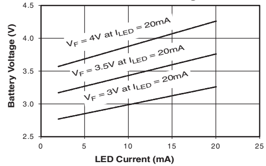
Upper Mode Charge Voltage vs LED Forward Voltage
