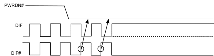
Figure 8. PWRDN# Assertion
