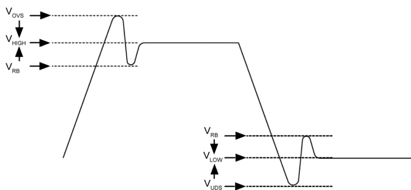
Figure 3. Single-Ended Measurement Points for V_{\text{OVS}} , V_{\text{UBS}} , and V_{\text{RB}}
