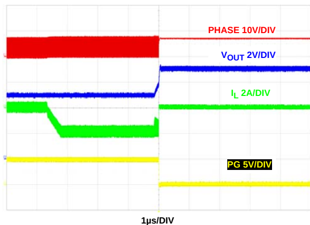
FIGURE 39. OVERVOLTAGE PROTECTION
