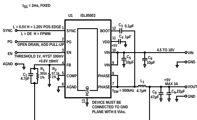
FIGURE 1A. ISL85003 V_{IN} RANGE FROM 4.5V TO 18V, V_{OUT} = 5V AND INTERNAL COMPENSATION WITH EXTERNAL FREQUENCY SYNC
