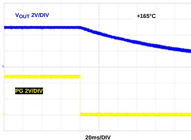
FIGURE 40. OVER-TEMPERATURE PROTECTION
