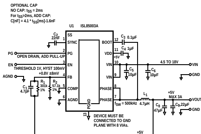
FIGURE 1B. ISL85003A V_{IN} RANGE FROM 4.5V TO 18V, V_{OUT} = 5V AND INTERNAL COMPENSATION WITH EXTERNAL SOFT-START
