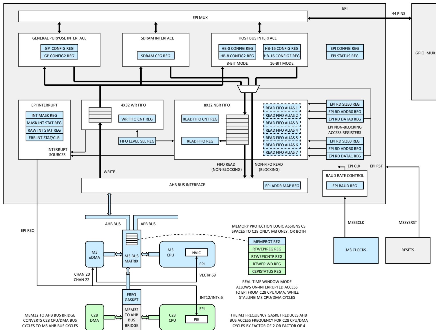
Figure 7-7. EPI
