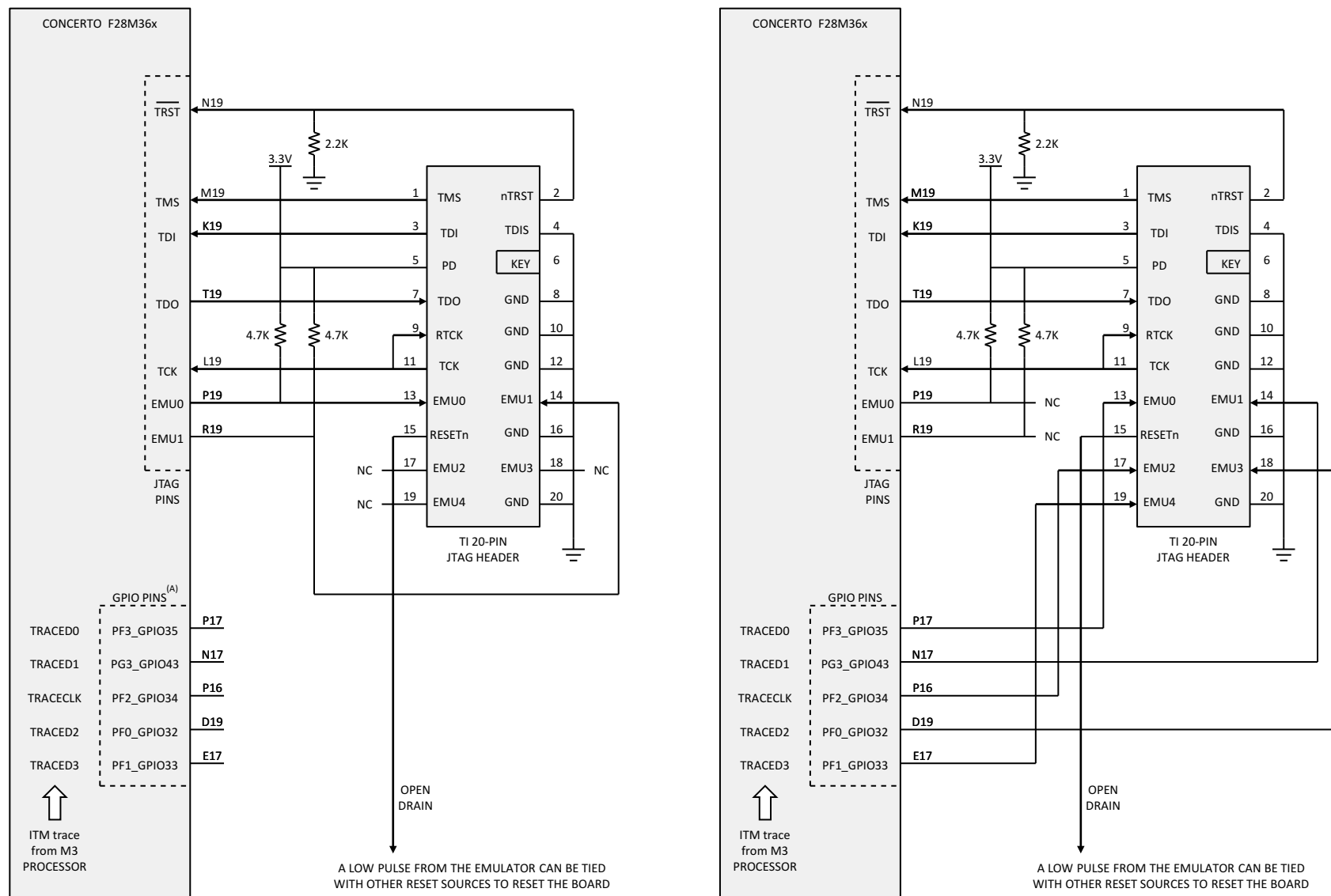
Figure 3-19. Connecting to TI 20-Pin JTAG Emulator Header
