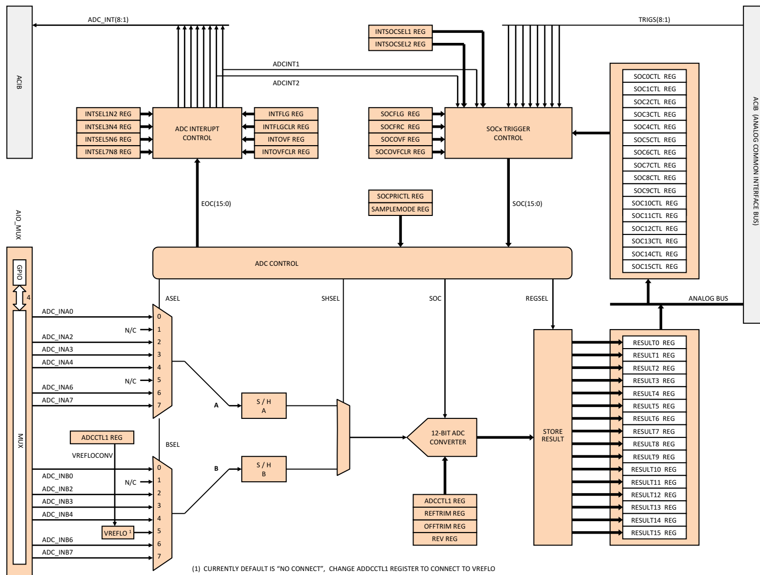
Figure 7-1. ADC
