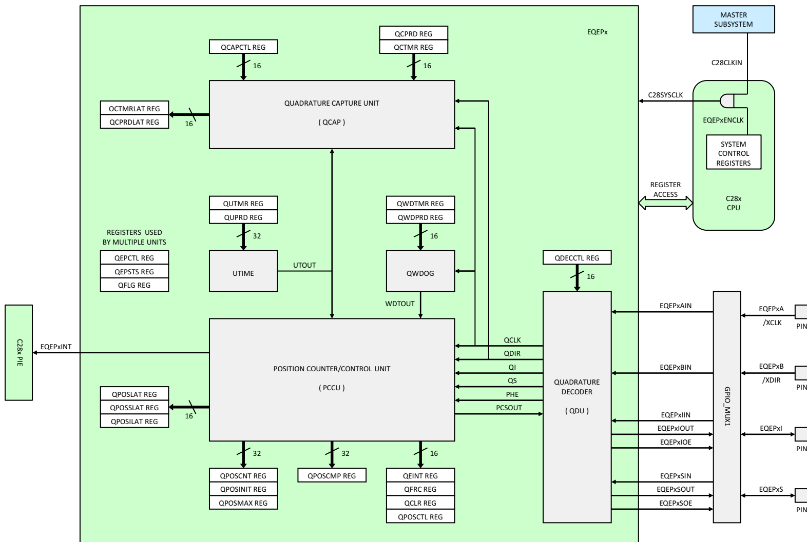
Figure 7-38. eQEP
