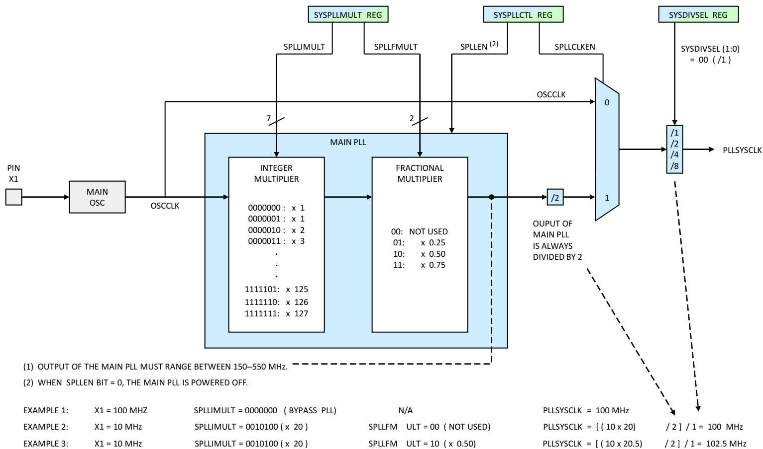
Figure 3-8. Main PLL
