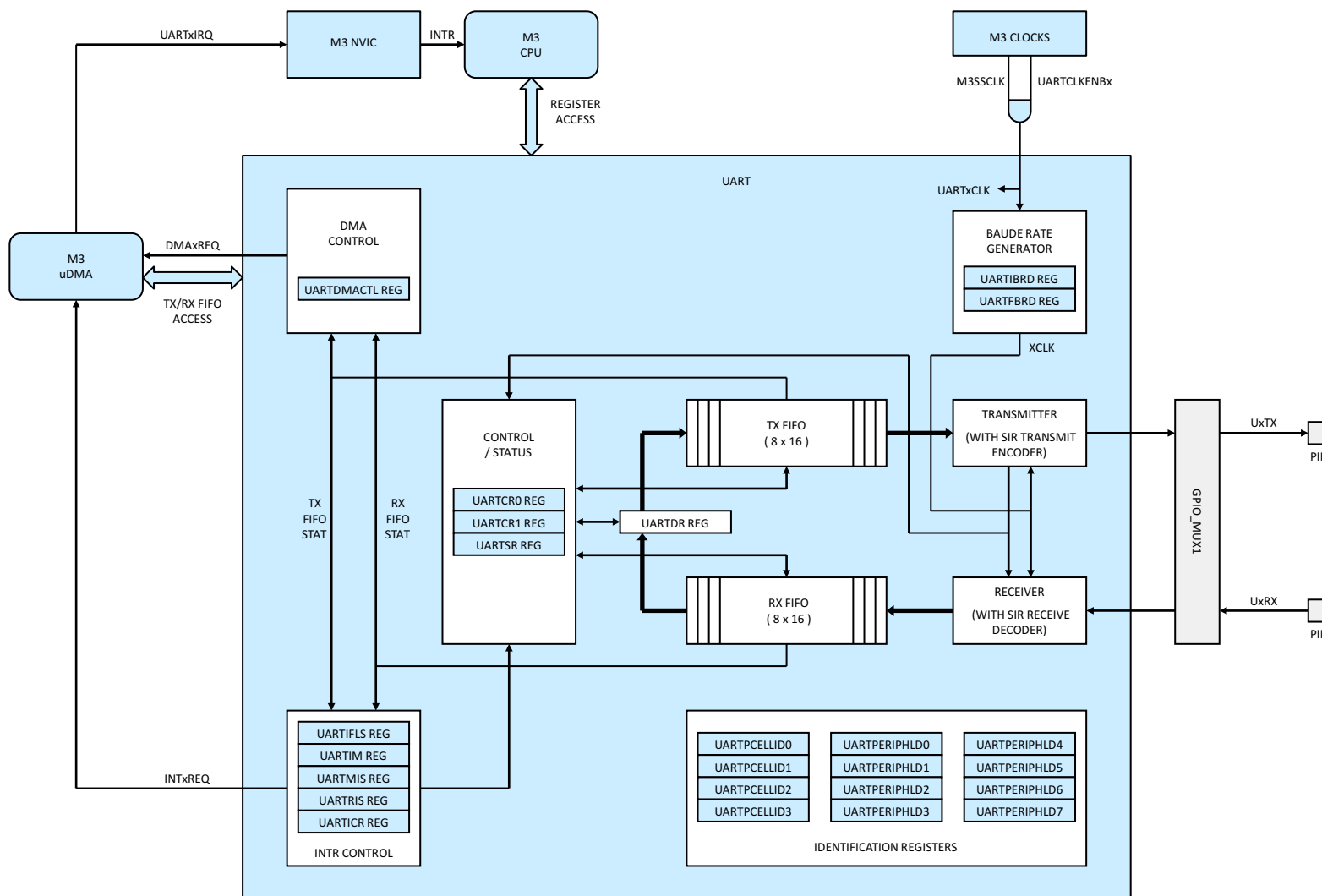
Figure 7-22. UART
