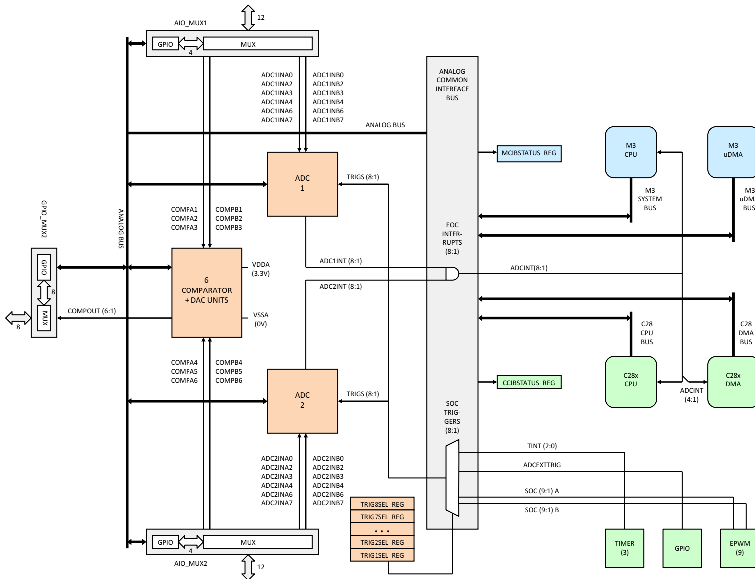
Figure 3-3. Analog Subsystem
