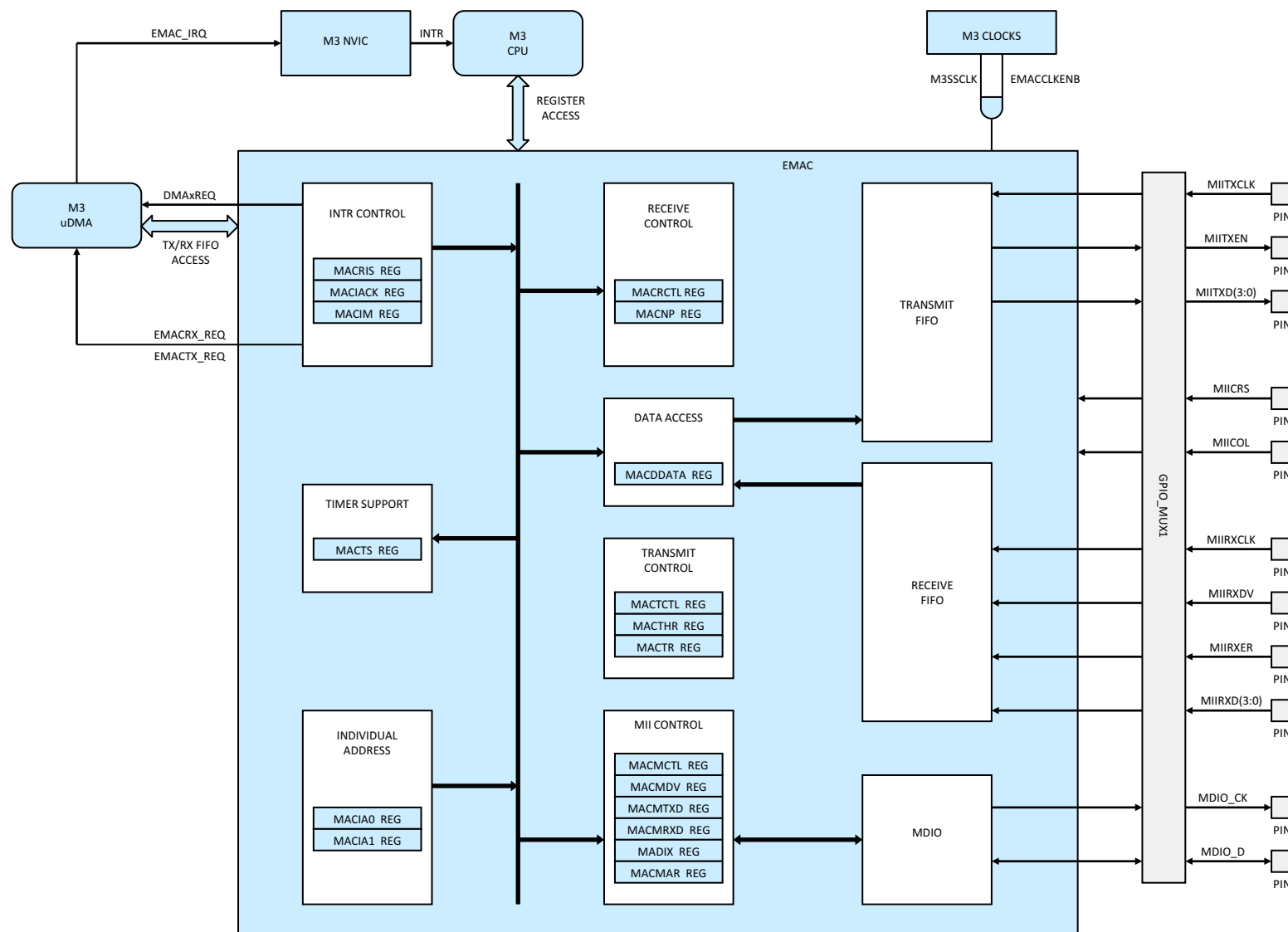
Figure 7-26. EMAC
