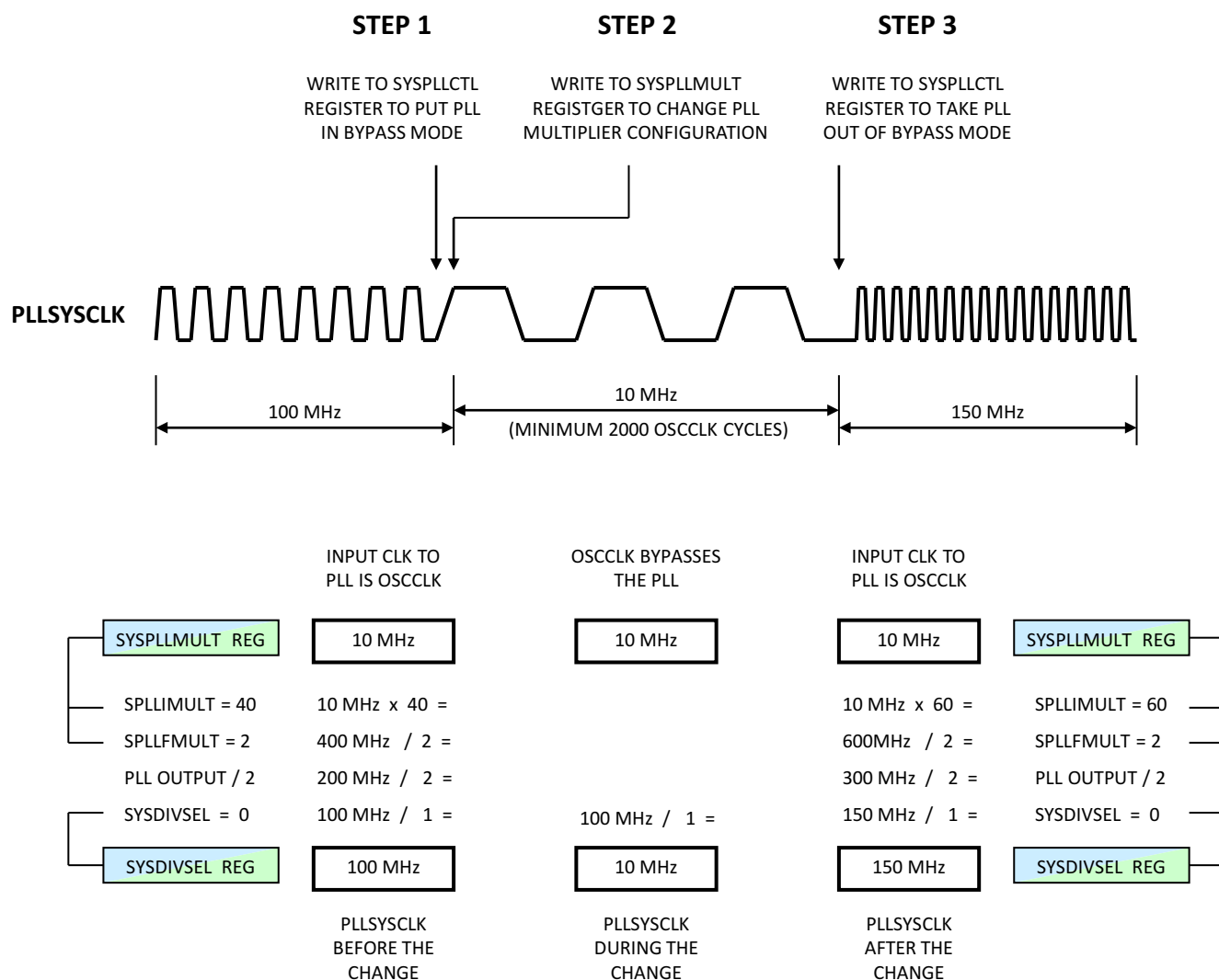
Figure 6-4. Changing the Frequency of the Main PLL
