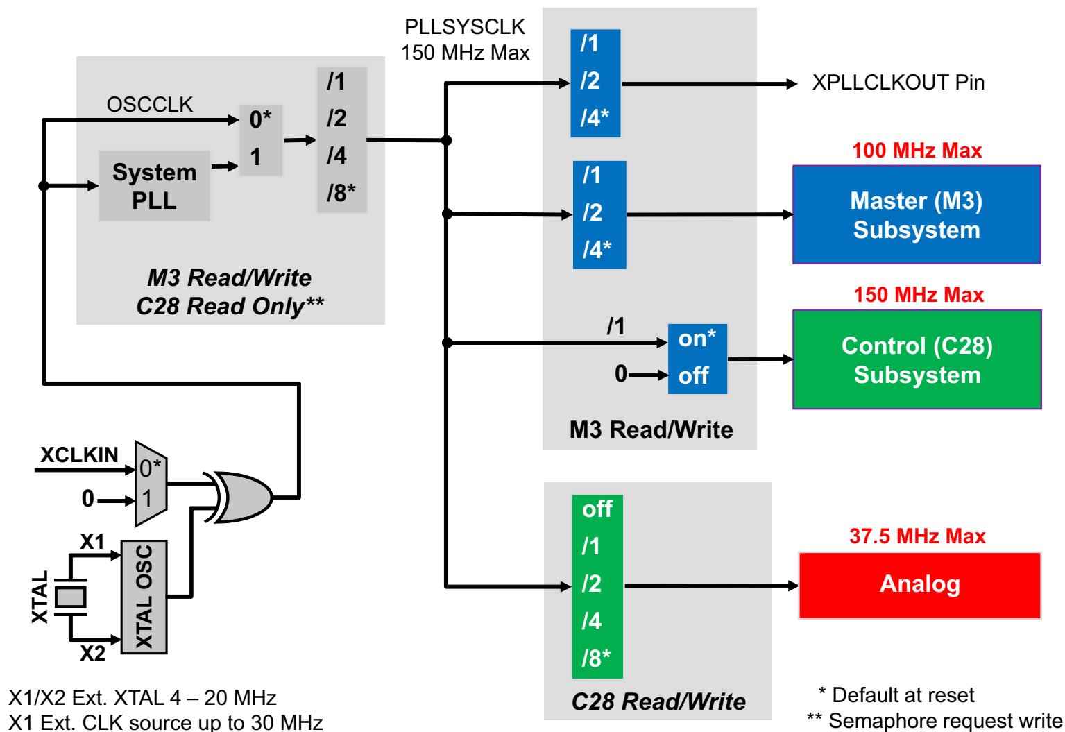
Figure 3-11. System Clock/PLL
