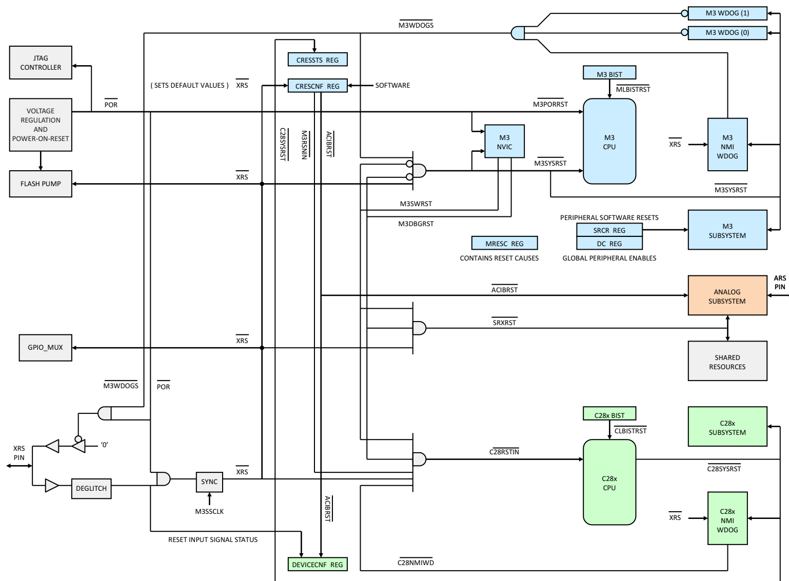
Figure 3-5. Resets
