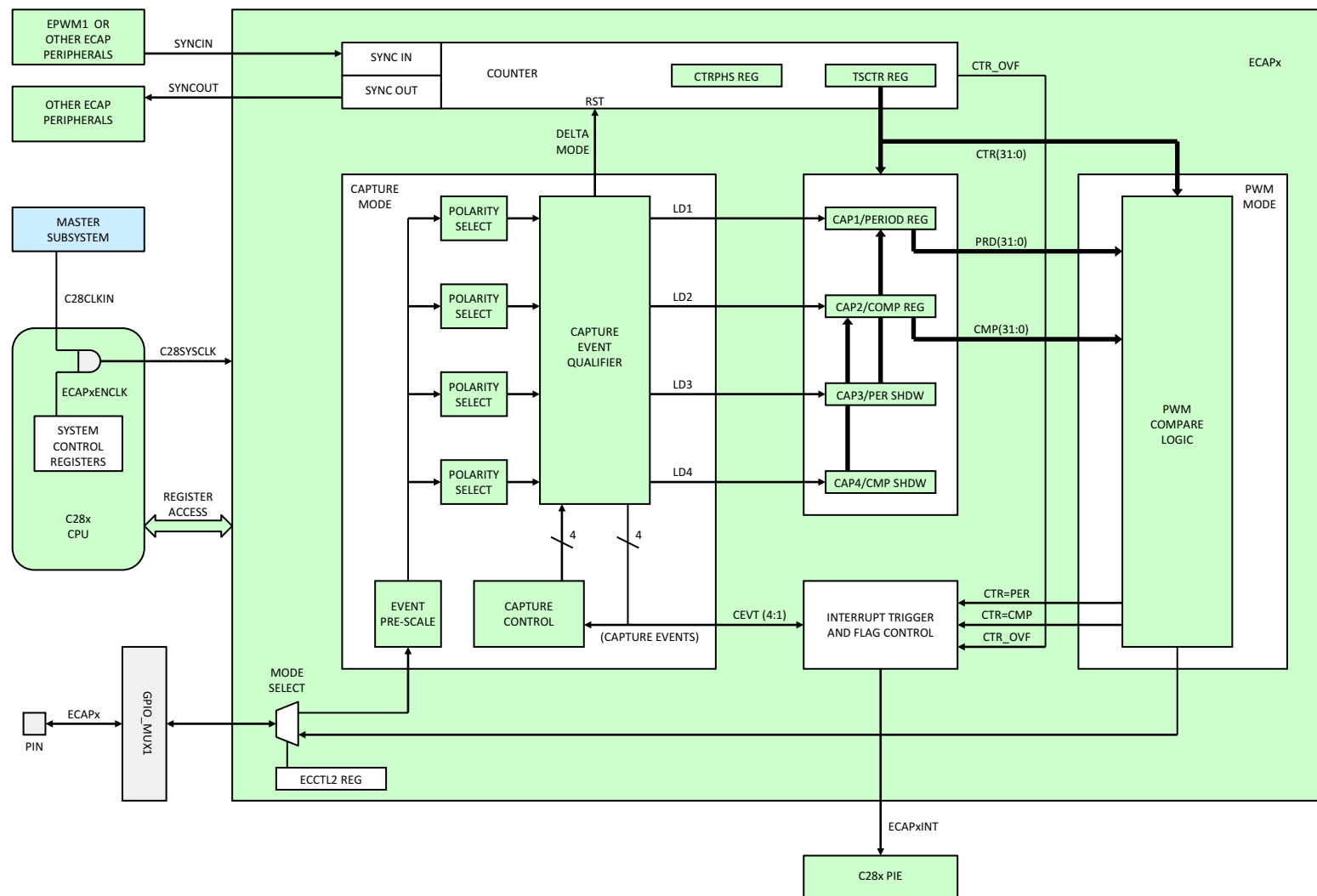
Figure 7-37. eCAP
