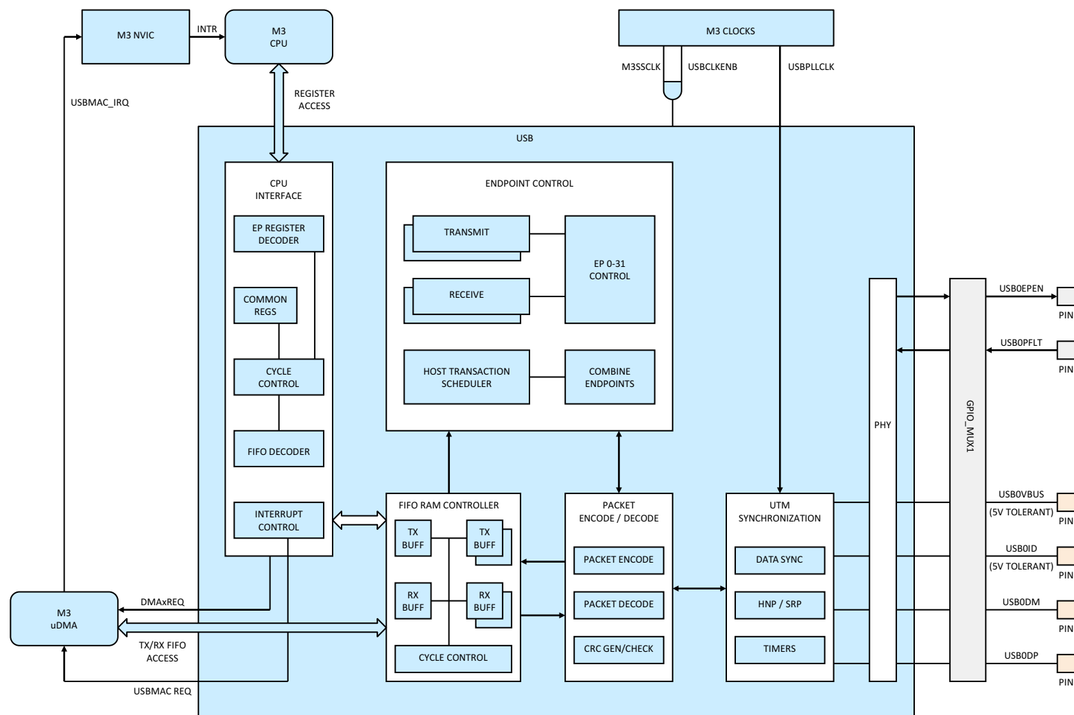
Figure 7-25. USB
