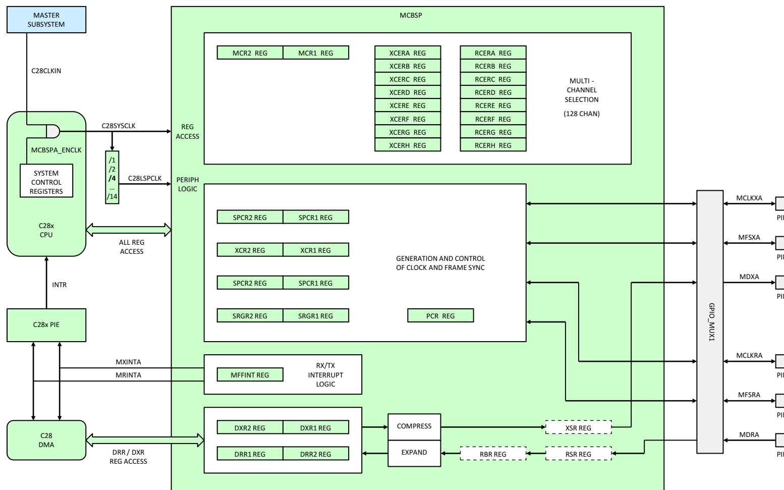
Figure 7-46. McBSP (C28x)
