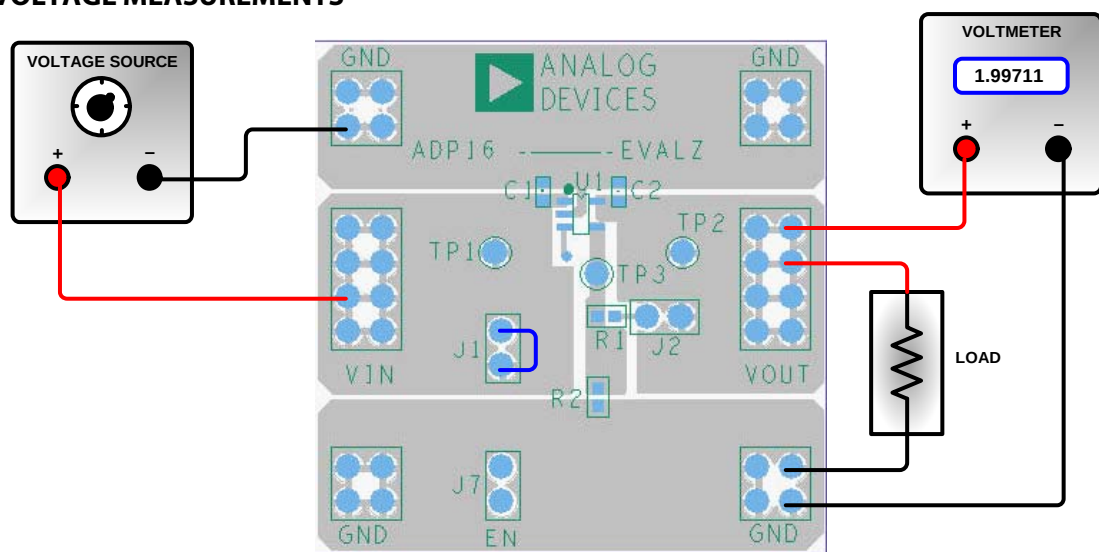
Figure 5. Output Voltage Measurement Setup, TSOT
