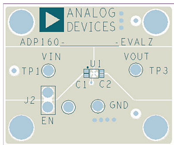
Figure 2. WLCSP PCB Layout
