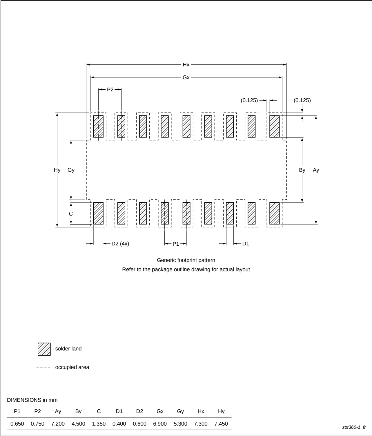
Footprint information for reflow soldering of TSSOP20 package
