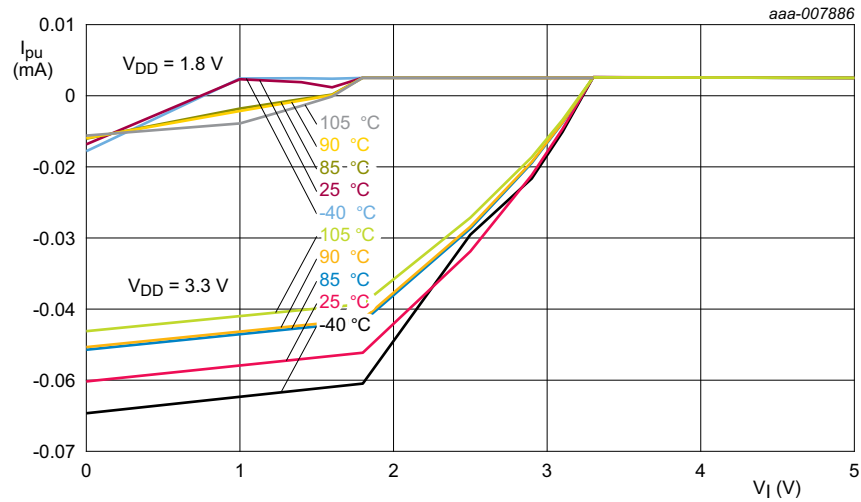
Fig 26. Typical pull-up current I_{pu} versus input voltage V_i
