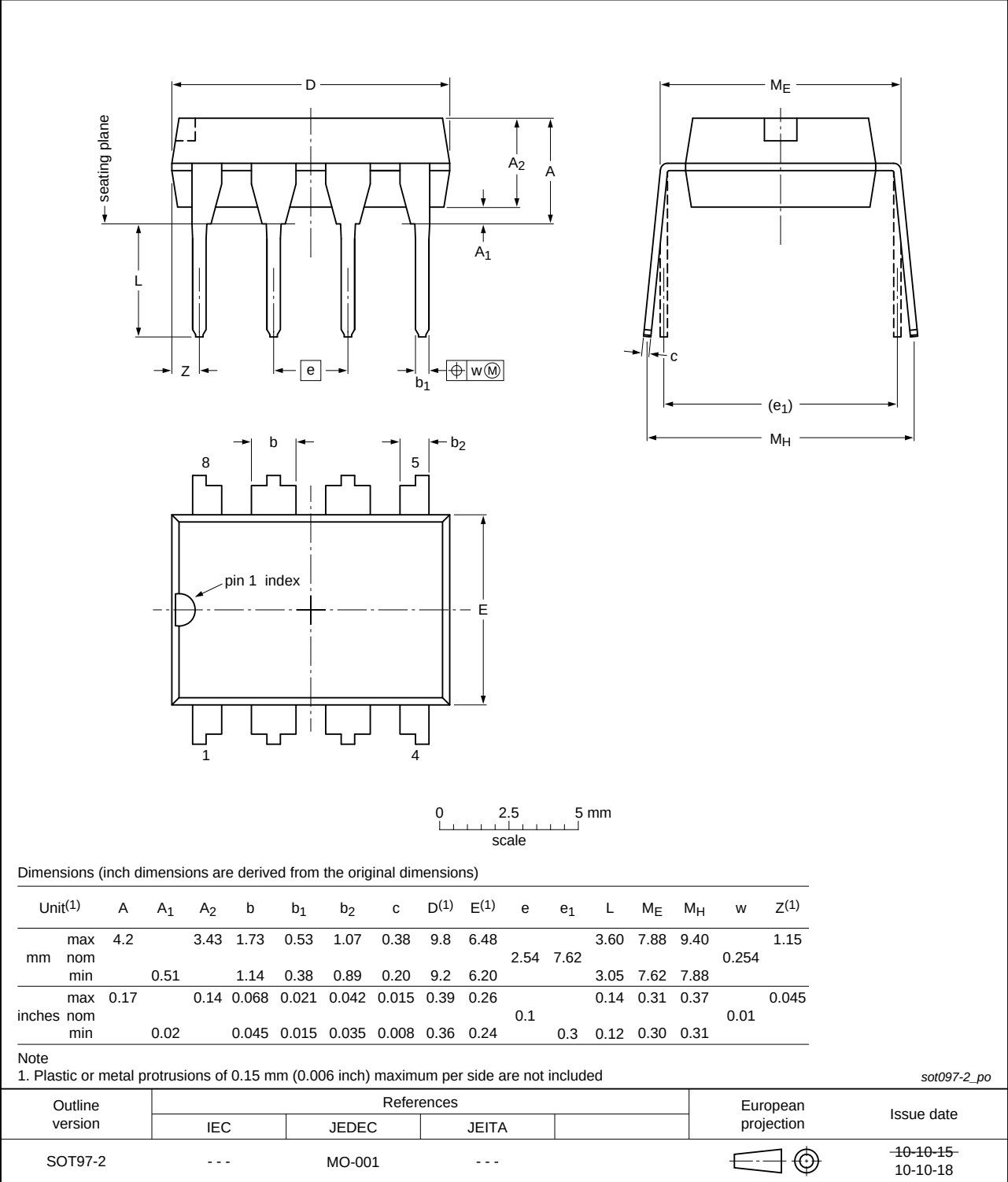
Fig 37. Package outline SOT097-2 (DIP8)
