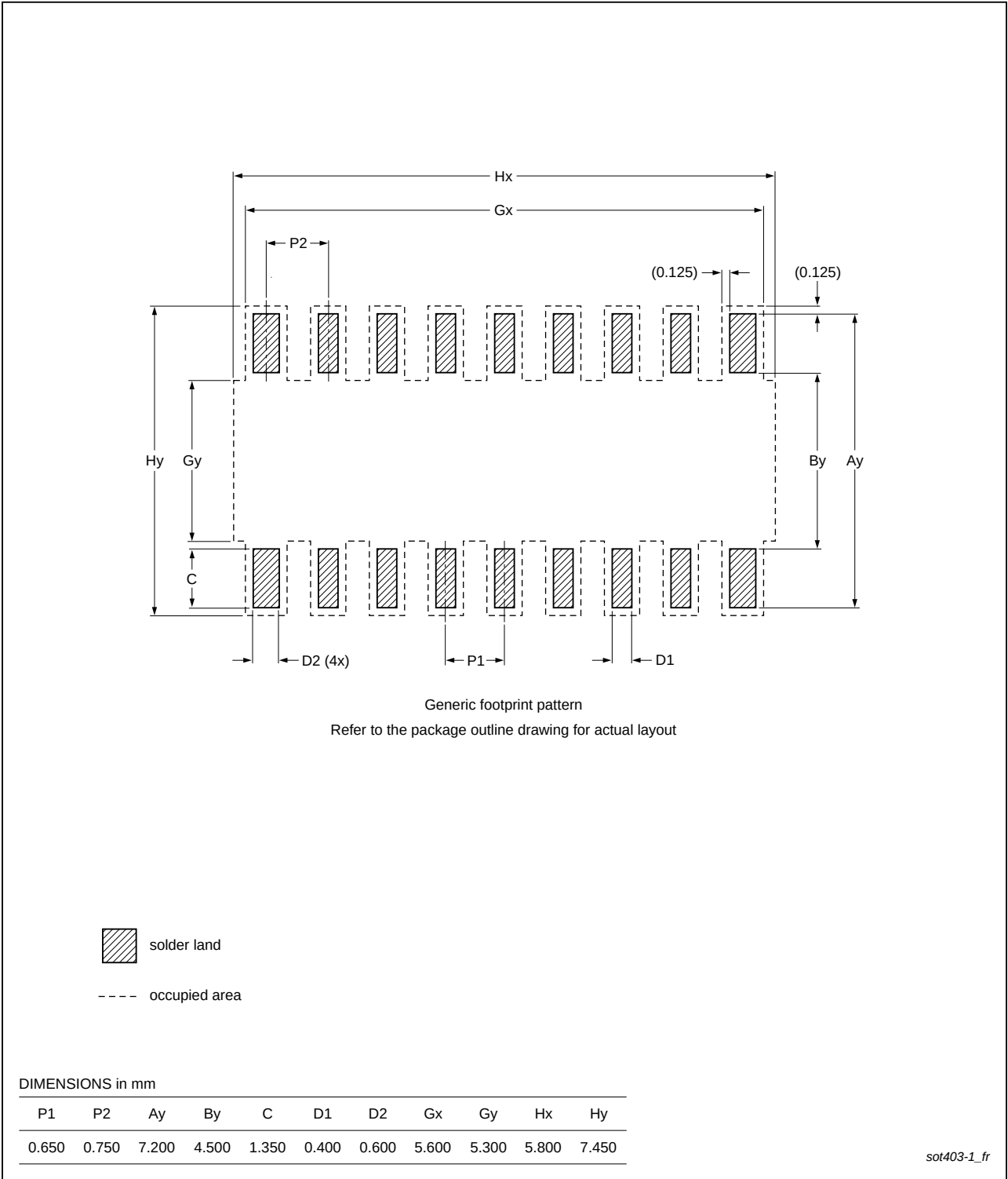
Fig 42. Reflow soldering of the TSSOP16 package
