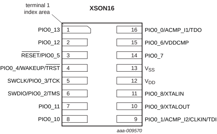
Fig 6. Pin configuration XSON16 package (LPC812M101JTB16)
