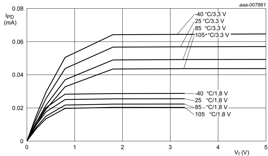
Fig 27. Typical pull-down current I_{pd} versus input voltage V_i
