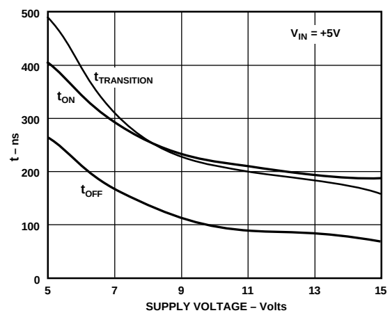
Figure 14. Switching Time vs. Single Supply
