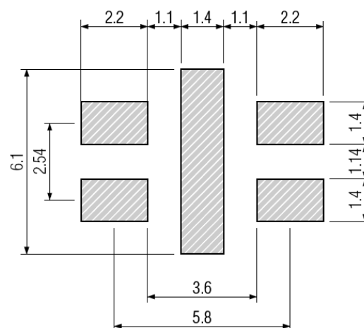
Figure 2) Land Pattern
