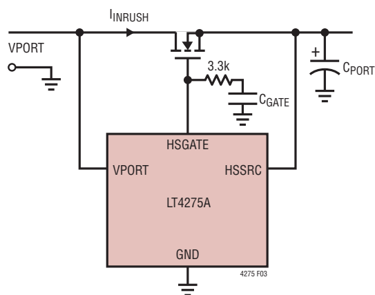
Figure 3. Programming I_{INRUSH}
