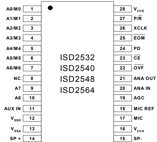
SOIC/PDIP
