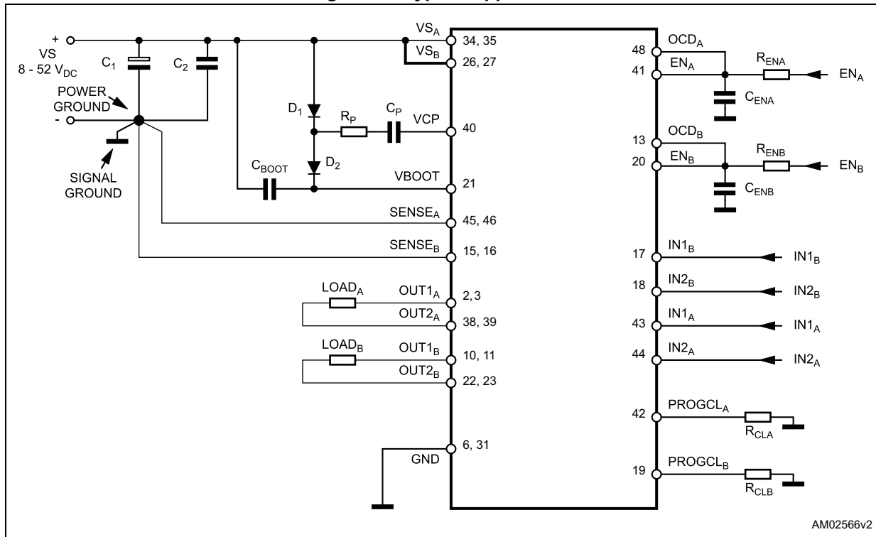
Figure 14. Typical application
