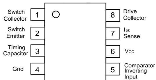
SO-8 ( Top View )
