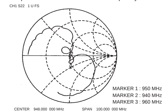
Output Reflection Coefficient vs. Frequency
