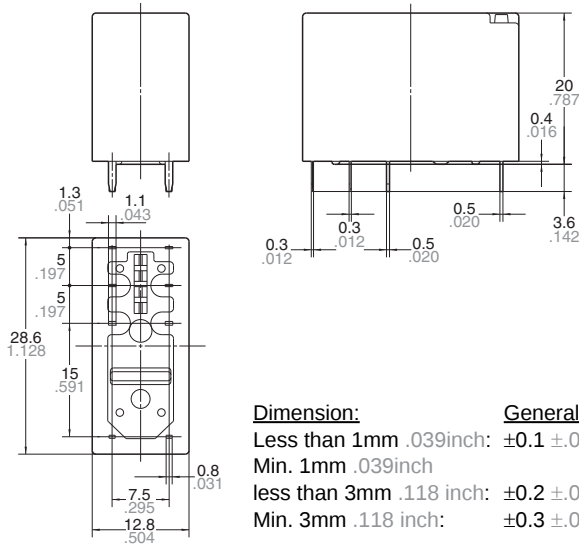
External dimensions
