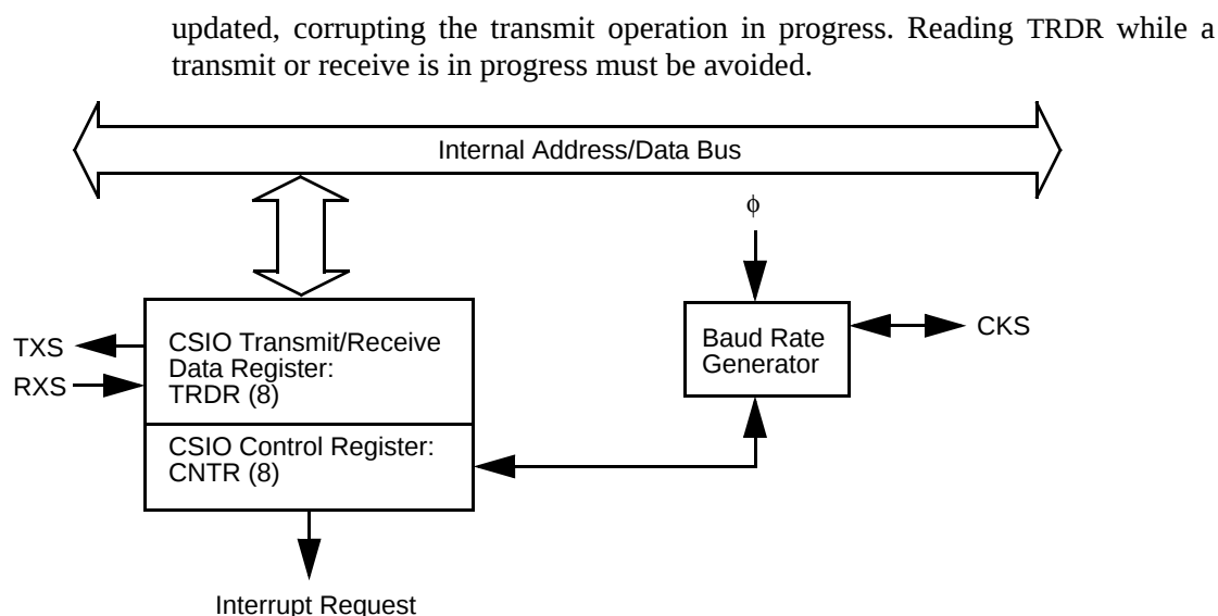
Figure 7. CSIO Block Diagram
