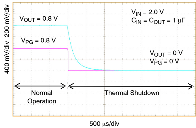
Figure 30. Turn-Off Response Due to Thermal Shutdown NCP752A/B, V_{OUT} = 0.8\text{ V}
