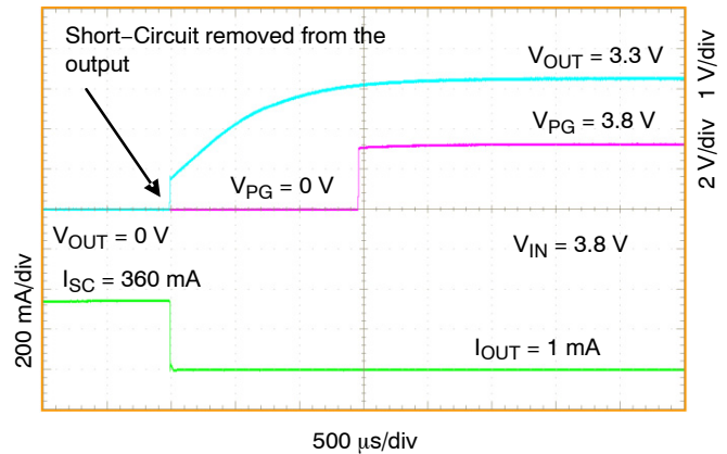
Figure 50. Recovery from Short-Circuit NCP752B, V_{OUT} = 3.3 V
