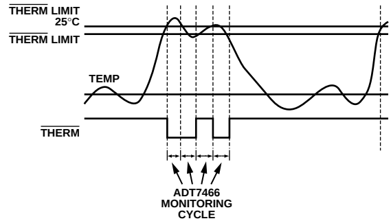
Figure 31. Asserting \overline{\text{THERM}} as an Output Based on Tripping \overline{\text{THERM}} Limits
