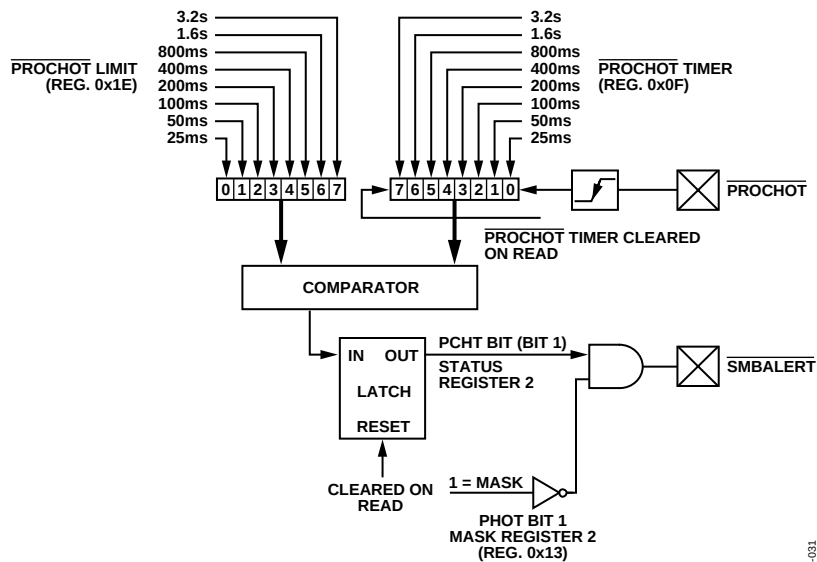
Figure 32. Functional Diagram of the ADT7466 \overline{\text{PROCHOT}} Monitoring Circuitry
