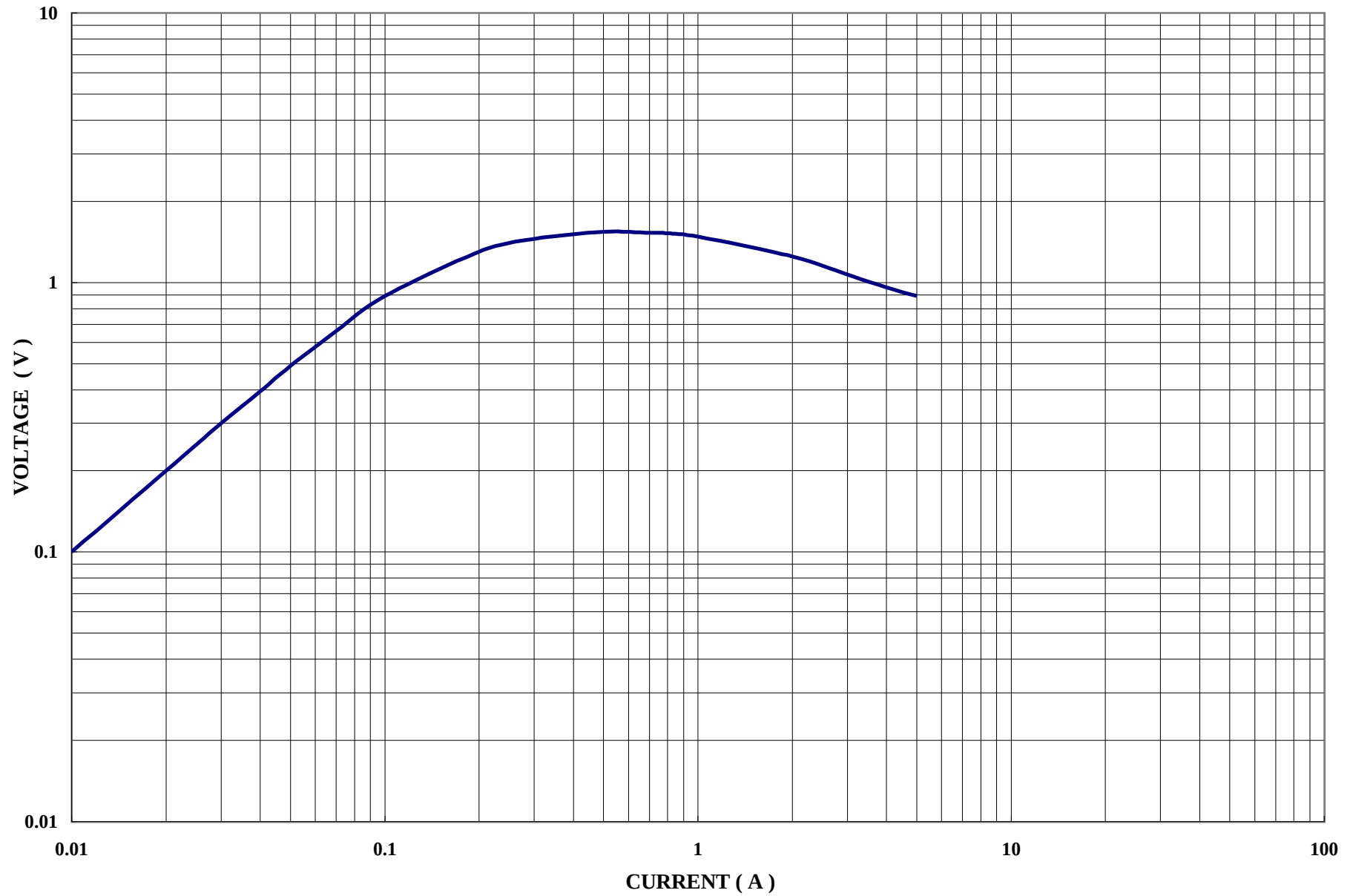
V-I Curve ( Nominal ) Part No. : N15SP010
