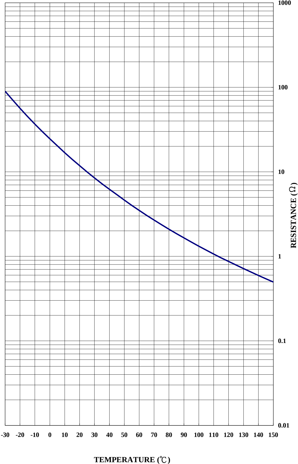
R-T Curve (Nominal) Part No : N15SP010
