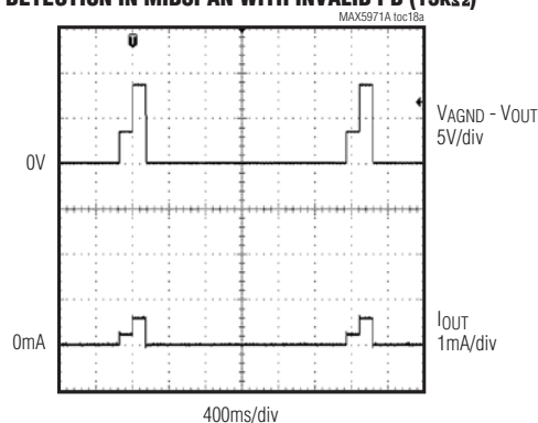
DETECTION IN MIDSPAN WITH INVALID PD (15kΩ)
